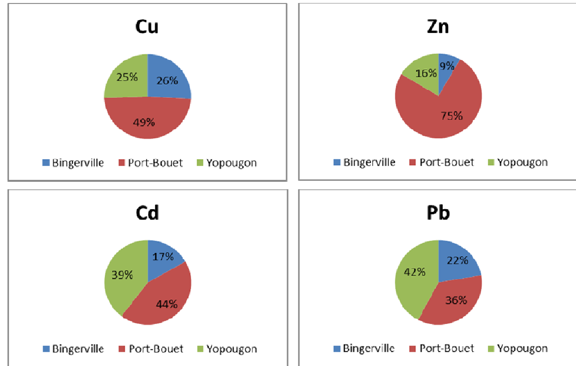
153 Fig.2. Proportion (%) of metal contents in topsoil (0 – 20 cm) as determined in vegetable growing 154 areas at Bingerville, Port-Bouët and Yopougon. 155
