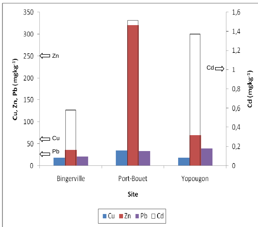
Fig.3: Mean values of soil contents of Cu, Zn, Pb and Cd in topsoil (0 – 20 cm) according the three sites studied (Moderate levels are pointed respectively)
