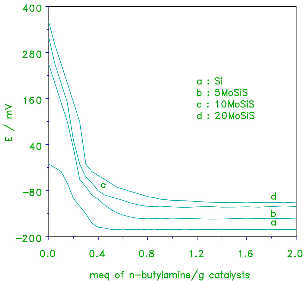
Fig. 2: Potentiometric titration curves of n-butyl amine in acetonitrile for the silica supported molybdena and sulfated catalysts (xMoSiS).
