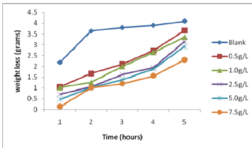
112 Fig 5: variation of weight loss with time for mild steel corrosion in 5 M H 2 SO 4 in the 113 presence and absence of ethanol extract of Alternanthera bettzickiana stem at 40 °C
