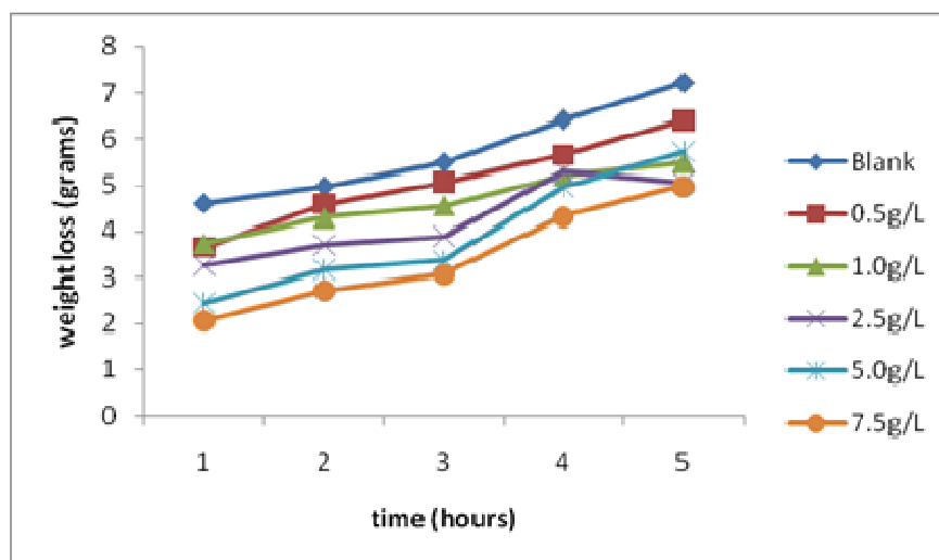
118 Fig 7: variation of weight loss with time for mild steel corrosion in 5 M H 2 SO 4 in the 119 presence and absence of ethanol extract of Alternanthera bettzickiana leaves at 60 °C.
