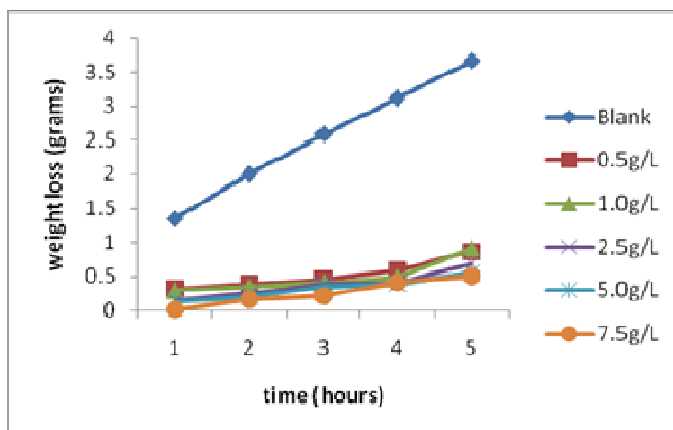
103 Fig 2: variation of weight loss with time for mild steel corrosion in 5 M H 2 SO 4 in the 104 presence and absence of ethanol extract of Alternanthera bettzickiana stem at 30 °C.
