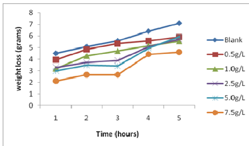
121 Fig 8: variation of weight loss with time for mild steel corrosion in 5 M H 2 SO 4 in the 122 presence and absence of ethanol extract of Alternanthera bettrockiana Stem at 60 °C.
