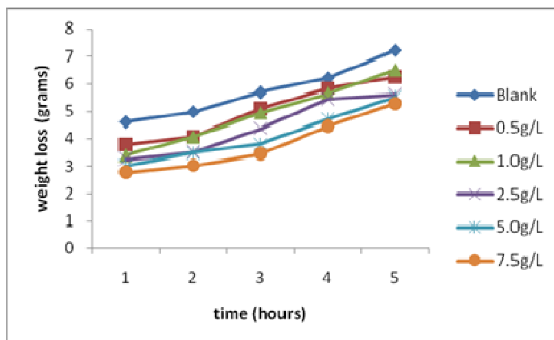
124 Fig 9: variation of weight loss with time for mild steel corrosion in 5 M H 2 SO 4 in the 125 presence and absence of ethanol extract of Alternanthera bettrockiana Root at 60 °C. 126
