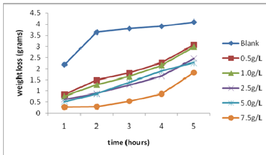
109 Fig 4: variation of weight loss with time for mild steel corrosion in 5 M H 2 SO 4 in the 110 presence and absence of ethanol extract of Alternanthera bettzickiana leaves at 40 °C.
