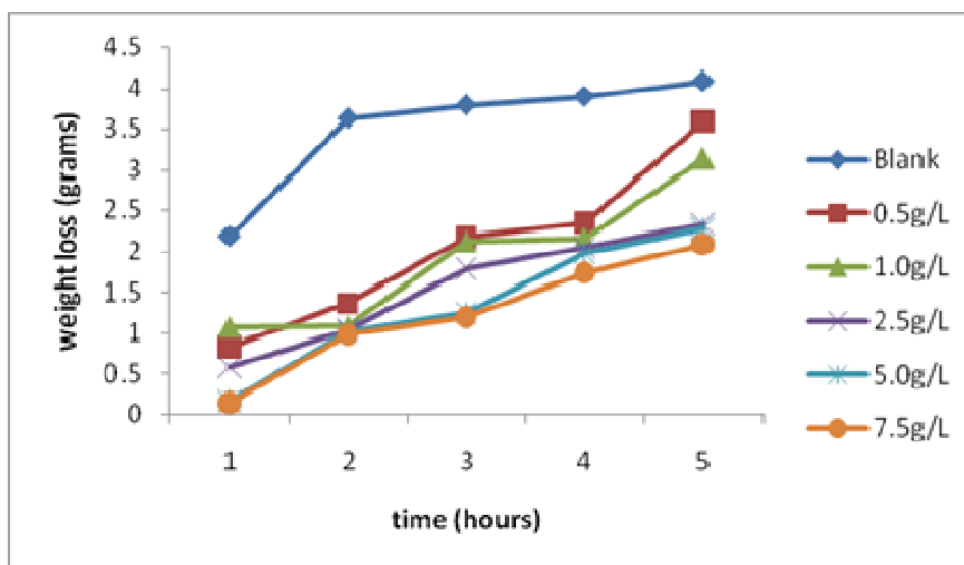
115 Fig 6: variation of weight loss with time for mild steel corrosion in 5 M H 2 SO 4 in the 116 presence and absence of ethanol extract of Alternanthera bettzickiana root at 40 °C.
