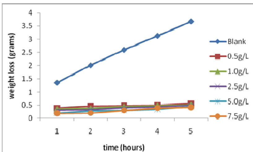
106 Fig 3: variation of weight loss with time for mild steel corrosion in 5 M H 2 SO 4 in the 107 presence and absence of ethanol extract of Alternanthera bettzickiana root at 30 °C.
