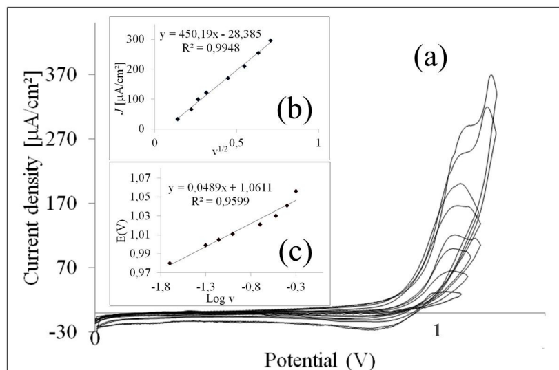
Figure 10. (a) Cyclic voltammetric responses of 5 \times 10^{-3} M LiClO 4 (0.1 M)/MeCN + 35mM HClO 4 at scan rate 0.02, 0.05, 0.07, 0.1, 0.2, 0.3, 0.4, 0.5 V.s -1 . (b) The plot of peak currents vs. root of scan rate. (c) The variation of potential vs. log v.
