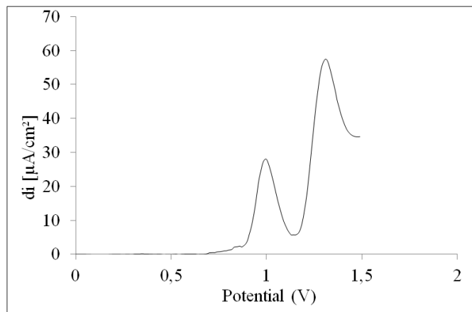
Figure 2. Square wave voltammogram of SIC ( 5 \times 10^{-3} M) in \text{Bu}_4\text{NBF}_4 (0.1 M)/MeCN; v = 100 mV/s; working electrode: GCE; reference electrode: Ag/AgCl
