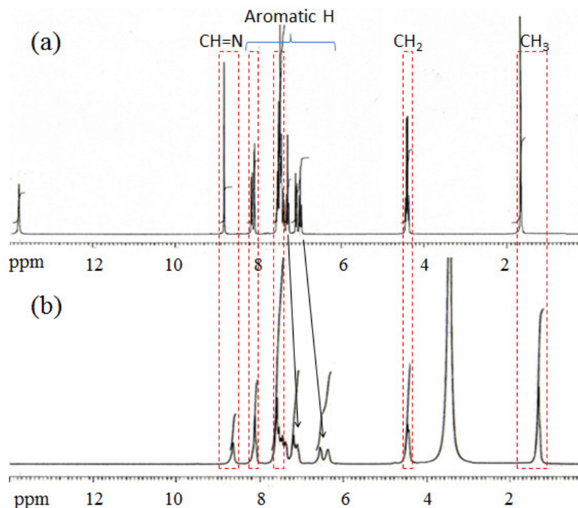
Figure 11. ^1\text{H} NMR spectrum of a) SIC , b) DIC .
