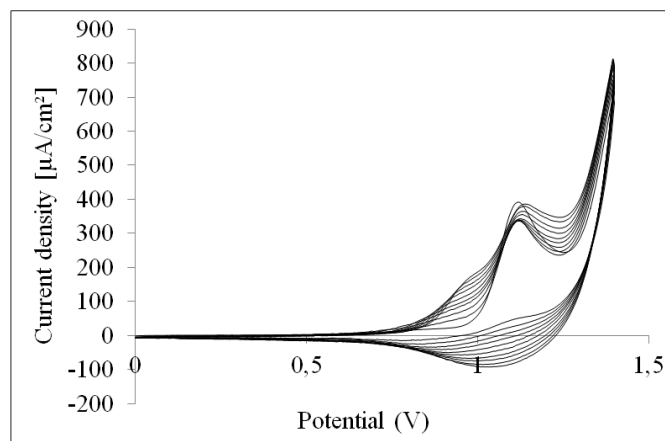
Figure 3. Electropolymerization of SIC ( 5 \times 10^{-3} M) in \text{Bu}_4\text{NBF}_4 (0.1 M)/MeCN; 10 sweeps between 0V and 1.4V; v = 100 mV/s; working electrode: GCE; reference electrode: Ag/AgCl
