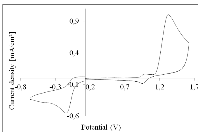
Figure 6. Cyclic voltammogram of SIC 5 \times 10^{-3} M in \text{LiClO}_4 (0.1 M)/MeCN + 35mM \text{HClO}_4 ; v = 100 mV/s; working electrode: GCE; reference electrode: Ag/AgCl
