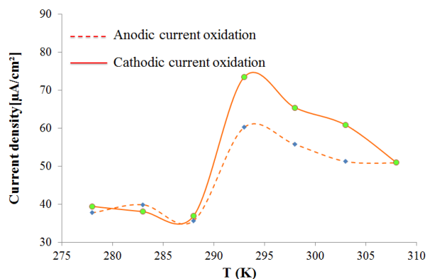
111 112 Figure 5. Influence of temperature on current density values measured at p-doping/undoping potential 113 of PDIC . (----) Anodic current density. (—) Cathodic current density.
