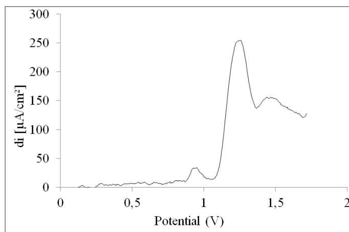
Figure 7. Square wave voltammogram of SIC 5 \times 10^{-3} M in \text{LiClO}_4 (0.1 M)/MeCN + 35mM \text{HClO}_4 ; v = 100 mV/s; working electrode: GCE; reference electrode: Ag/AgCl
