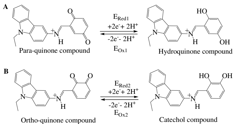
Scheme 3. Redox behaviour of: A) Para -quinone compound, B) Ortho -quinone compound.
