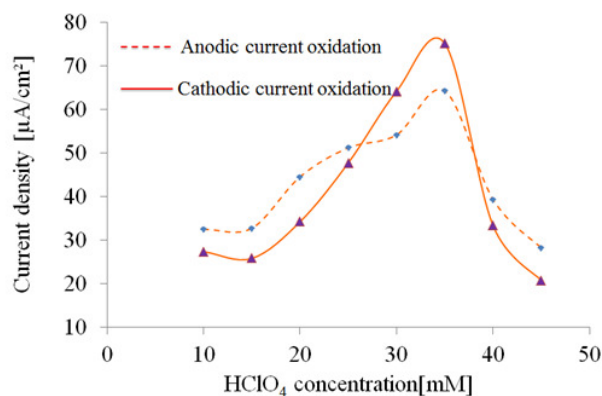
104 Figure 4. Influence of \text{HClO}_4 concentration on current density measured at p-doping/undoping 105 potential of PDIC . (----) Anodic current density. (—) Cathodic current density. 106
