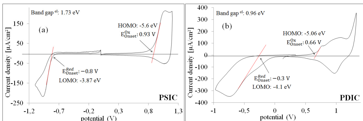
214 Figure 13. Cyclic voltammograms for oxidation of: a) PSIC coated GCE in \text{Bu}_4\text{NBF}_4 (0.1 M)/MeCN; 215 b) PDIC coated GCE in \text{LiClO}_4 (0.1 M)/MeCN + 35mM \text{HClO}_4 . v = 100\text{mV/s} .
