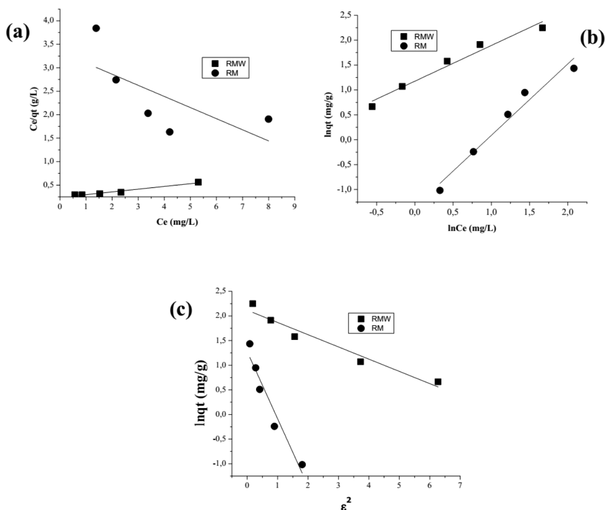
Fig. 9. (a) Langmuir, (b) Freundlich and (c) Dubinin Radushkevich isotherms plots for MB removal on RMW and RM
