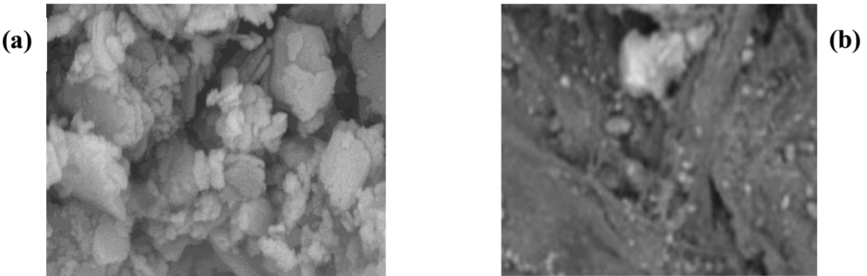
Fig. 2. SEM images of (a) RM (300nm) and (b) RMW (250 μm)
