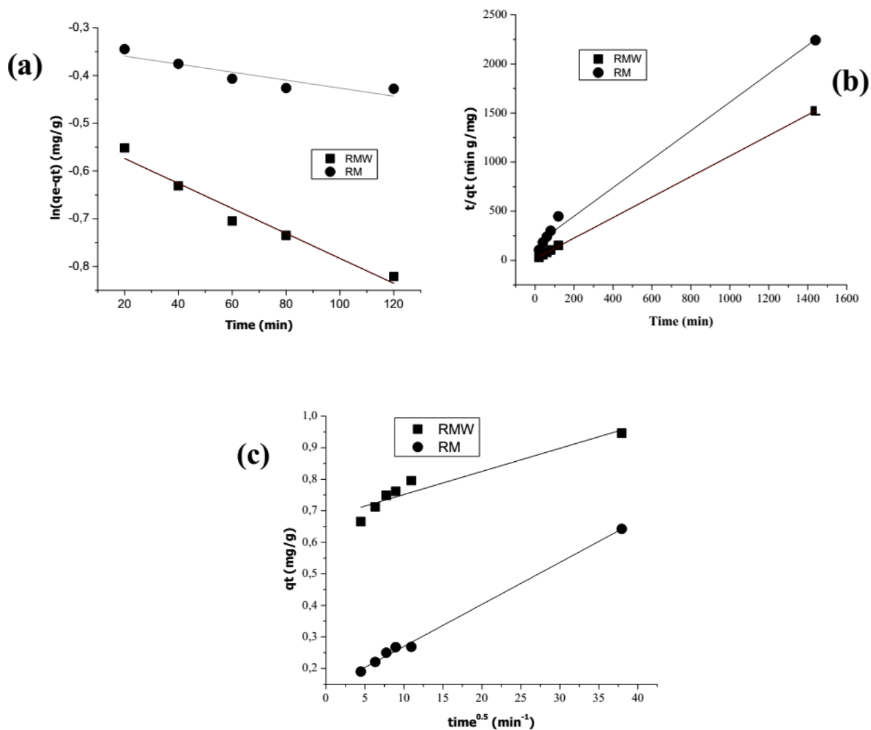
Fig. 10. (a) Pseudo-first order, (b) pseudo-second order and (c) intraparticle diffusion models kinetic plots for MB removal on RMW and RM
