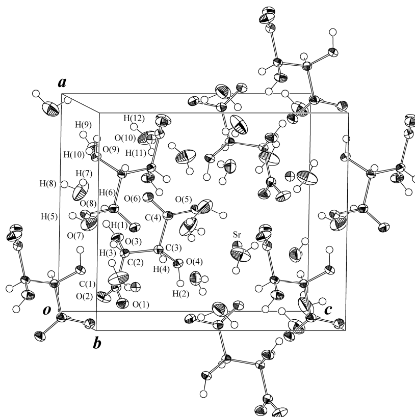
Fig. 1. Perspective view of the \text{SrC}_4\text{H}_4\text{O}_6 \cdot 4\text{H}_2\text{O} structure at room temperature with 50% probability-displacement thermal ellipsoids
