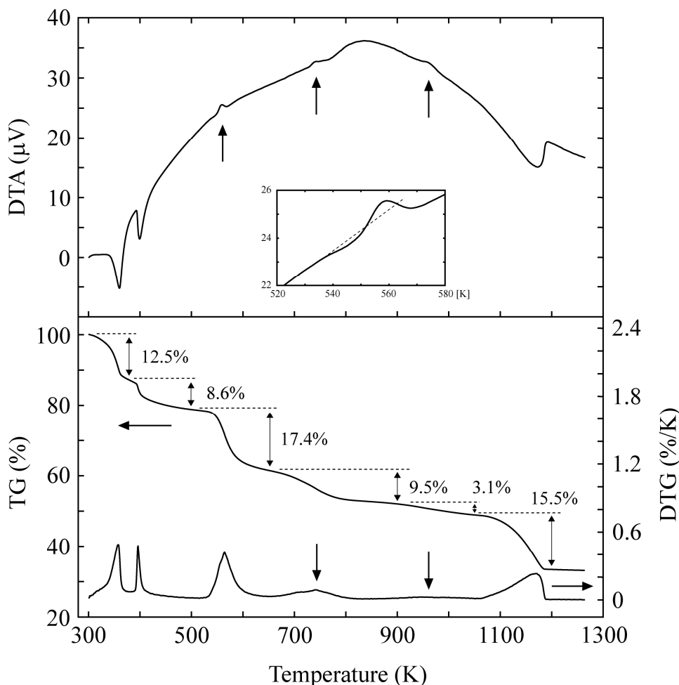
332 Fig. 3. TG, DTG, and DTA thermograms for the \text{SrC}_4\text{H}_4\text{O}_6 \cdot 4\text{H}_2\text{O} crystal on heating. The 333 inset figure shows an enlarged view of the curve around 550 K. The sample weight 334 (powder) was 3.46mg, and the heating rate was 10 \text{ K min}^{-1} under a dry \text{N}_2 flux of 300 335 \text{ml min}^{-1} .
