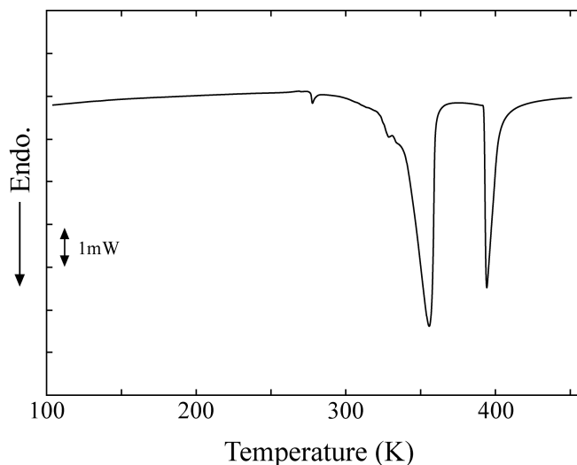
Fig. 2. DSC curve for the \text{SrC}_4\text{H}_4\text{O}_6 \cdot 4\text{H}_2\text{O} crystal on heating. The sample weight (powder) was 3.32 mg, and the heating rate was 5 K/min under a dry \text{N}_2 flux of 40 ml \text{min}^{-1} .
