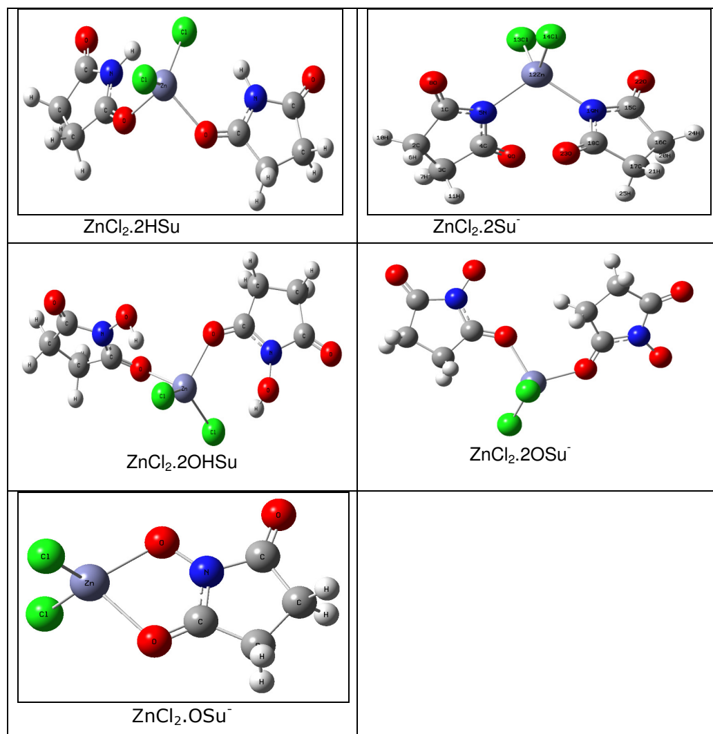
Fig.2. Structure of the modeled complexes
