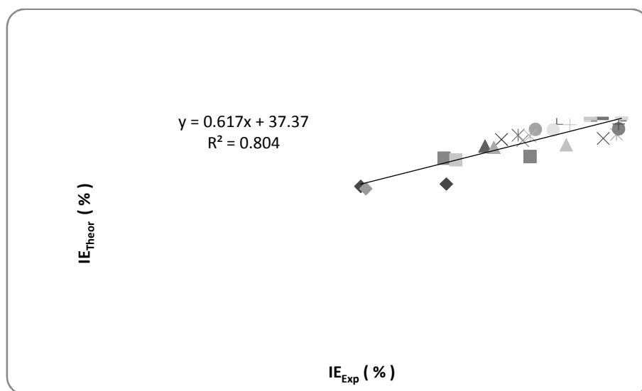
Figure 4. Plot of calculated inhibition efficiencies ( IE_{Theor} ) obtained from equation (4) versus experimental inhibition efficiencies ( IE_{Exp} )
