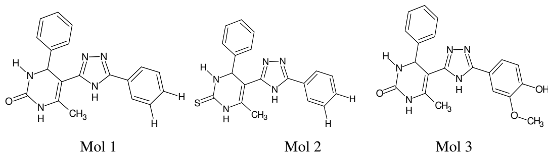
Figure 1. Chemical structure of Inhibitors (mol 1 and 3. Triazole pyrimidinones, mol 2. Triazolopyrimidine thione)
