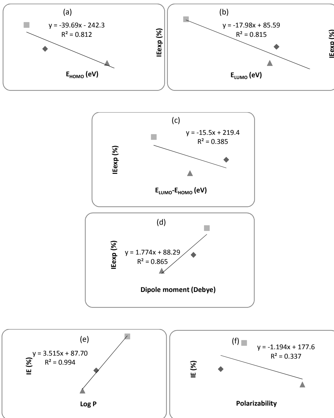
Figure 3. Variation of experimental inhibition efficiency (IE exp ) of the studied Triazolopyrimidines with (a) E_{HOMO} (b) E_{LUMO} (c) E_{LUMO} - E_{HOMO} (d) Dipole moment (e) Log P and (f) Polarizability obtained from AM1 calculations
