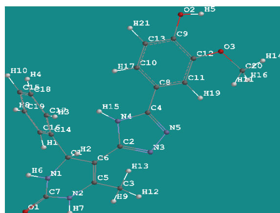
Figure 2. Optimised structure of Inhibitors (mol 1 and 3. Triazole pyrimidinones, mol 2. Triazolopyrimidine thione)
