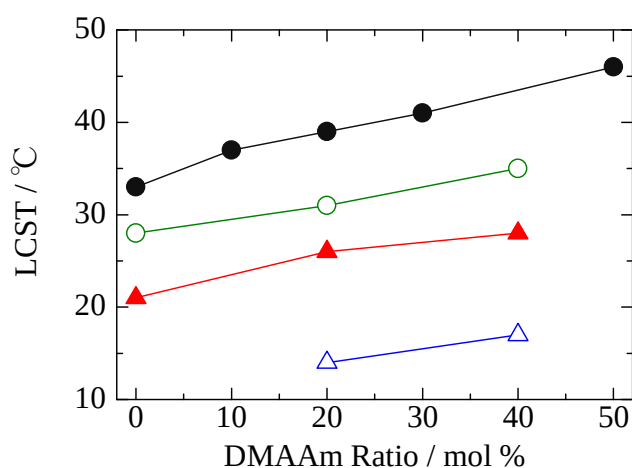
Fig. 6. LCSTs observed for NIPAAm-co-BA-co-DMAAm as a function of DMAAm ratios. In this figure, ratios of DMAAm are plotted as a function of total amount of NIPAAm and BA (ratios of NIPAAm:BA are 1.00:0.00 (●), 0.95:0.05 (○), 0.90:0.10 (▲), and 0.80:0.20 (△), respectively).
