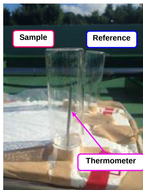
Fig. 3. Photograph of apparatus used for measuring temperatures in glass bottles outdoors.
