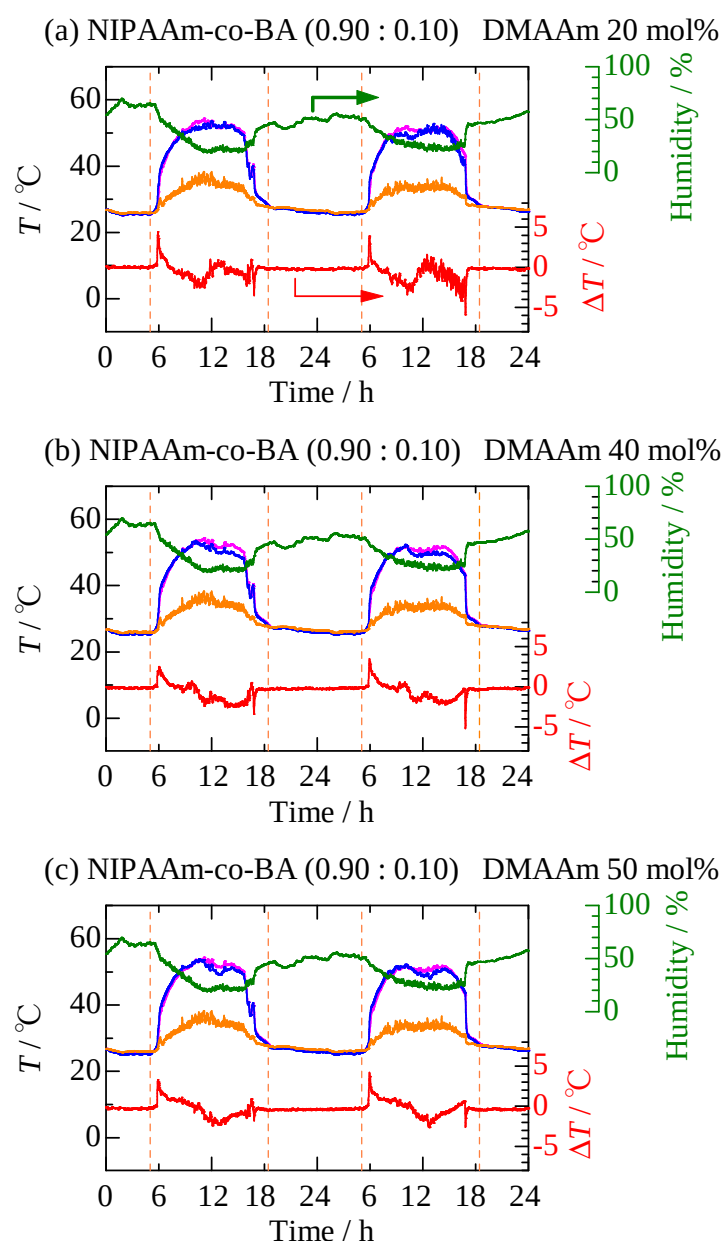
Fig. 7. Temperature changes in glass bottles coated with copolymer of NIPAAm-co-BA-co-DMAAm. DMAAm concentrations of (a) 20, (b) 40, and (c) 50 mol% relative to total amount of NIPAAm and BA with a mole ratio of 0.90:0.10. Temperatures of outer environment, reference, and sample are shown by orange, purple, and blue solid-lines, respectively. Temperature difference between sample and reference, and humidity are displayed by red and green curves. In this figure, sunrise and sunset times are shown by orange dotted lines.
