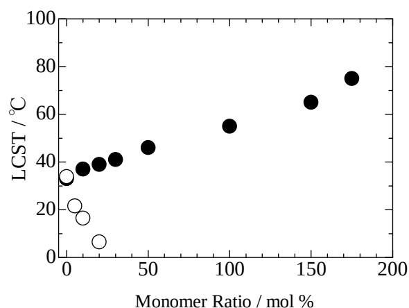
Fig. 5. Monomer ratio dependences of LCSTs observed for aqueous solution of NIPAAm-co-DMAAm(●) and NIPAAm-co-BA(○).
