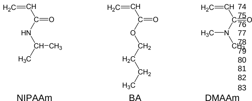
Fig. 1. Chemical structures of N-isopropylacrylamide (NIPAAm), butyl acrylate (BA), and N,N-dimethylacrylamide (DMAAm).
