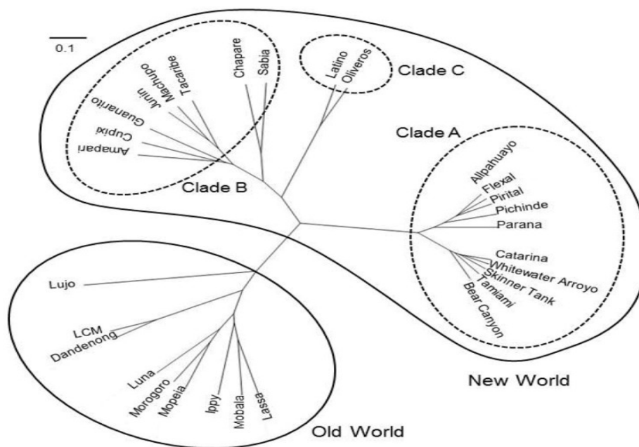
Figure 2: Phylogenetic tree of arenavirus Z protein. Amino acid sequences of Z protein were used for analysis.
