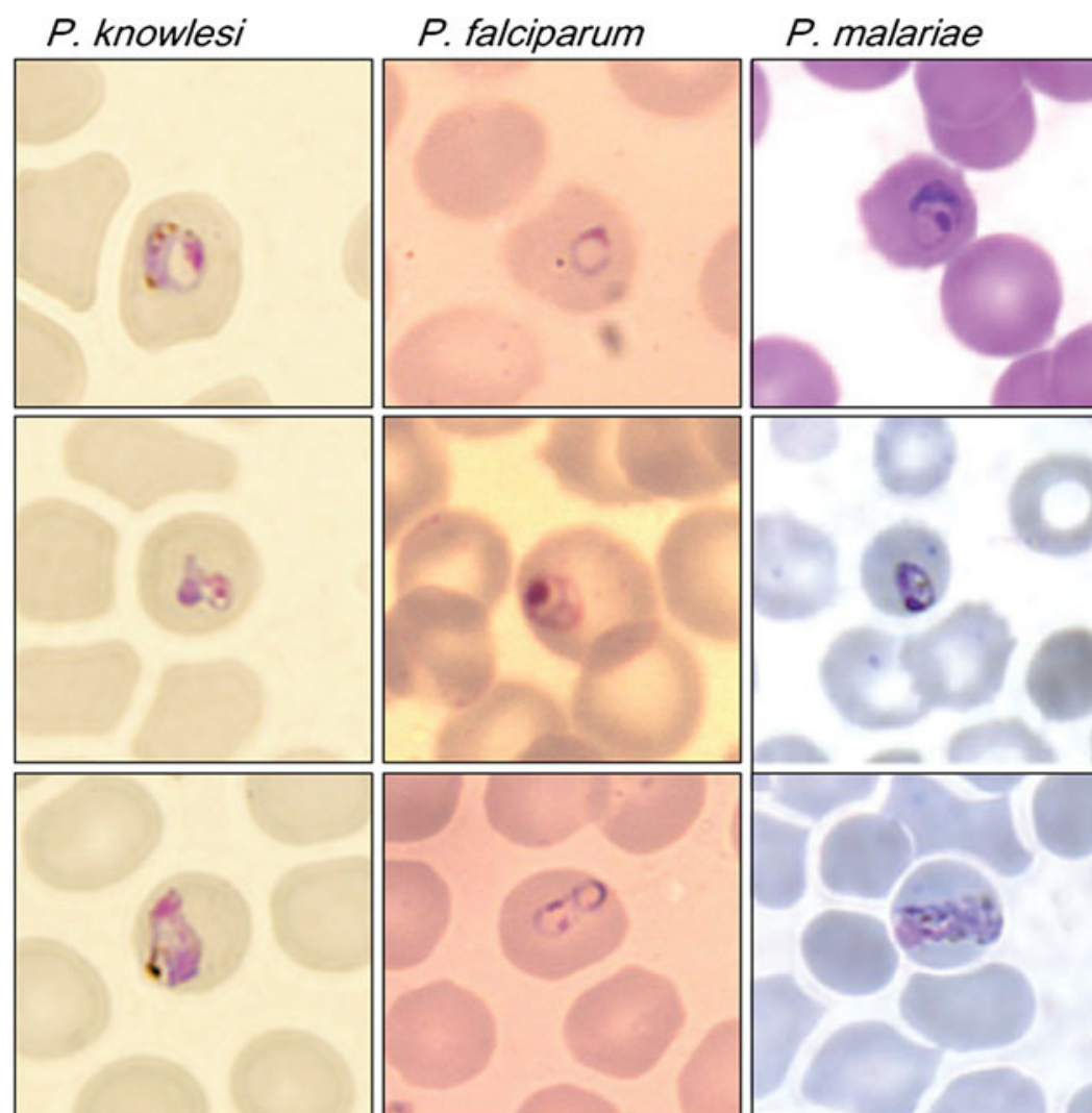
Fig 1: Morphologic forms of different types of Plasmodium with similar features as seen during microscopic examination
