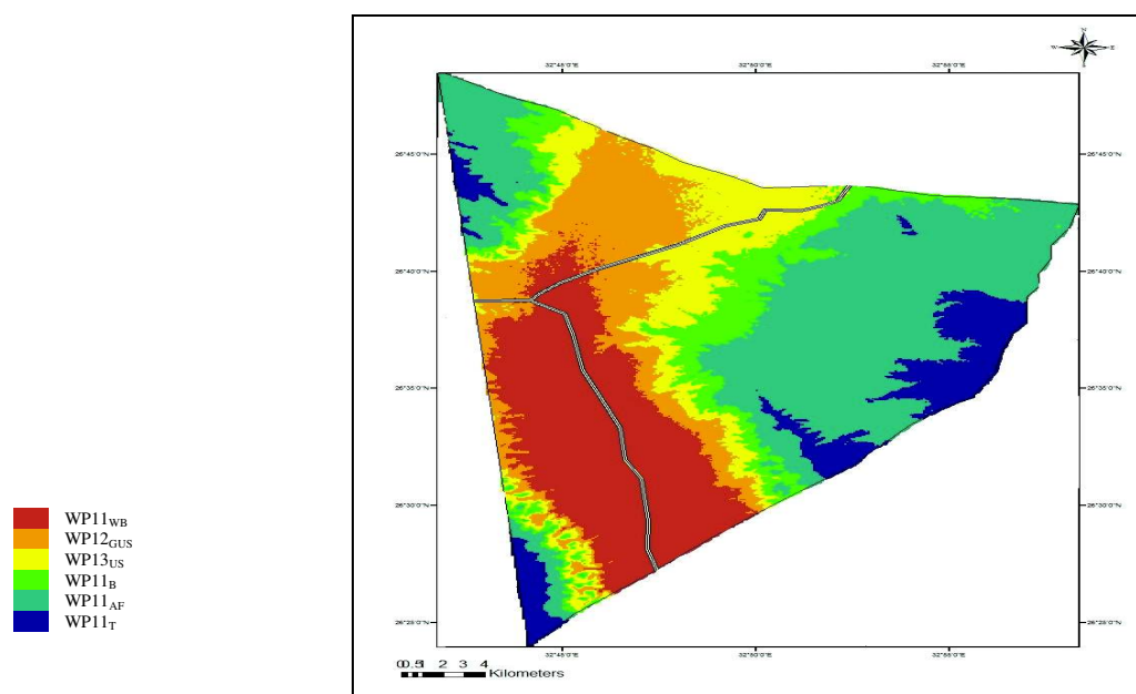
Fig. 6 Physiographic units map of the study area
