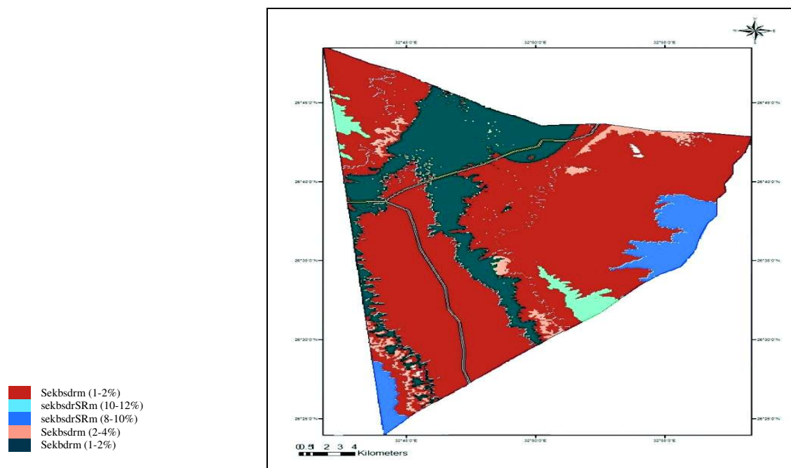
Fig.7 Fertility capability classification (FCC) units of the study area
