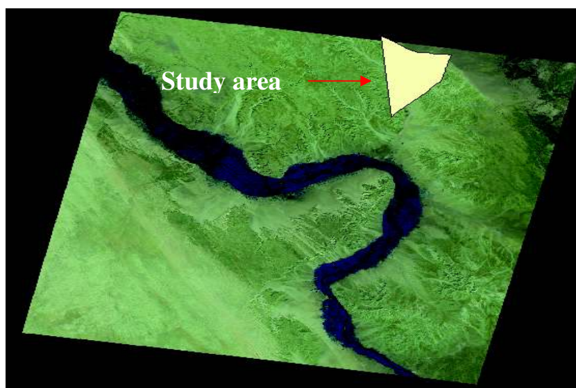
Fig.2 FCC of Landsat image of the studied area
