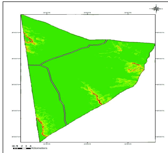
Fig.5 Slope map of the study area
