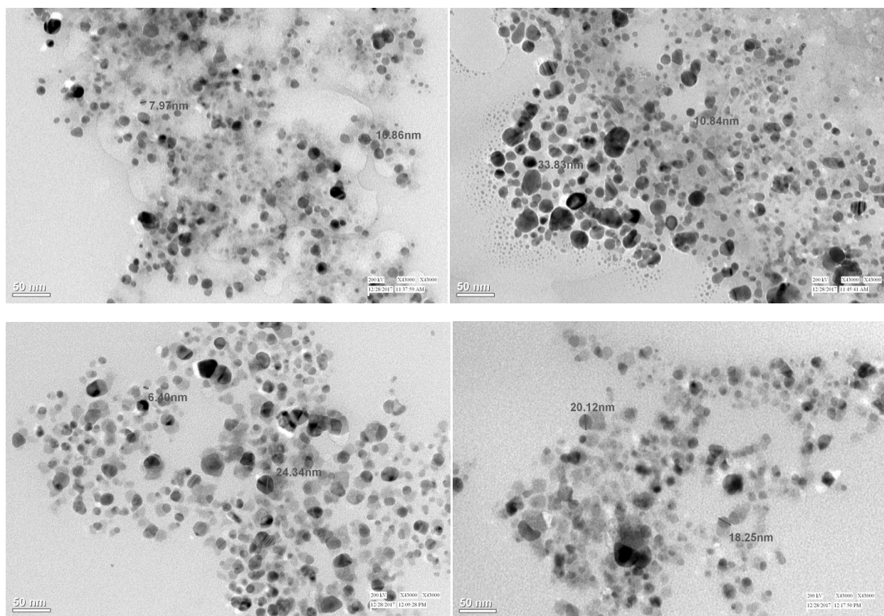
Figure: 11, 12, 13 and 14- Characterized AgNPs of aqueous and methanolic extracts of A. bisporus with different concentration (0.2g/ml and 0.4g/ml) by TEM analysis.
