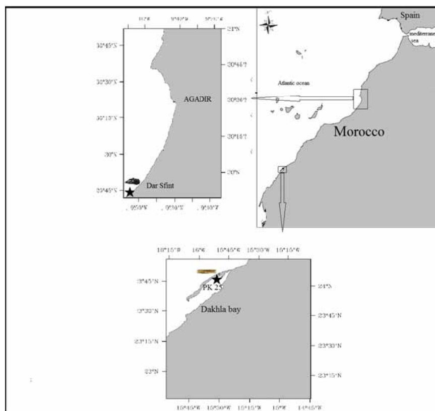
Figure 2. Sampling sites
