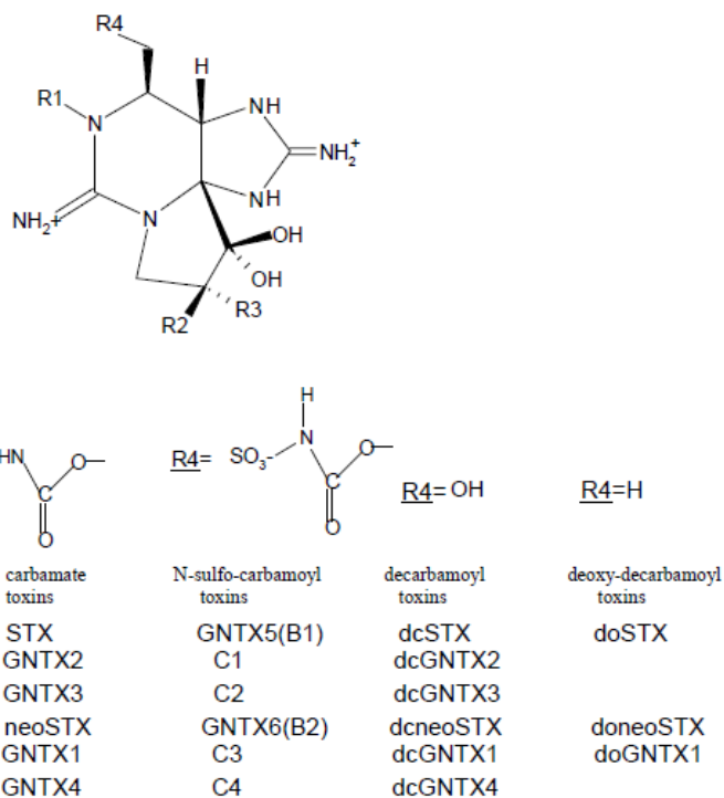
Figure 1: Chemical structures of PSP toxins
