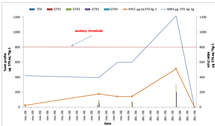
Figure 8: PSP by MBA and HPLC with toxines profile of Dakhla's solen during toxic even of end 2006
