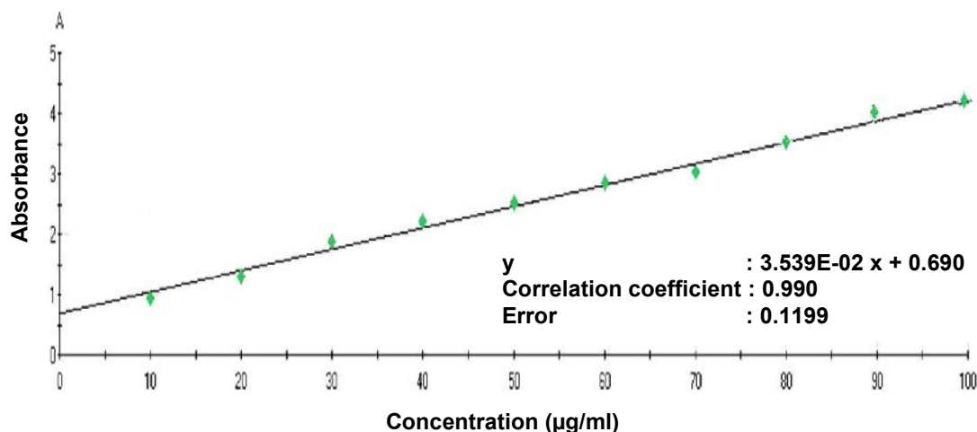
Figure 1. Total Phenolic Content (TPC): Calibration curve
