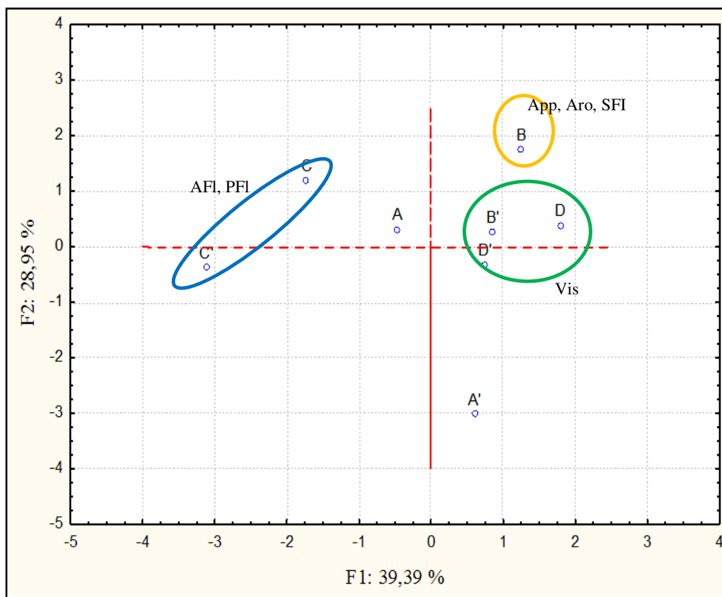
Fig 4: Distribution of the different MFPs dishes studied and their descriptors in the plan formed by the factors F1 and F2 of the principal components analysis
