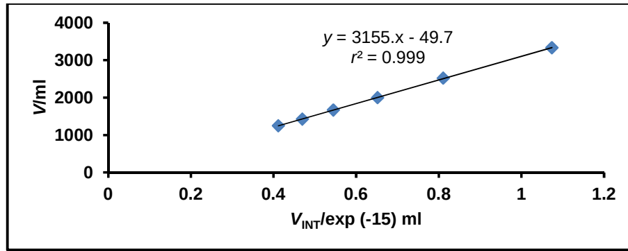
Fig. 2 The regression of volume ( V ) of the substrate solution on average interparticle volume ( V_{INT} ) for the determination of volume ( V_{\infty} ) at infinite dilution of the substrate concentration. V is volume of solvent in which the same mass of substrate is mixed to give any desired concentration; Total reaction mixture volume = 2ml. As shown in Eq. (12), I_{\infty} = 7.03 \pm 0.04 \exp(-7) m; V_{\infty} = 1.103 \pm 0.199 \exp(6) ml. Prepared [S] for assay ranges from 3 g/l – 8 g/l \equiv 10 g/3.333 l – 10 g/1.25 l (see Table 1 for detail); the concentration [S]_{\infty dil} at "infinite dilution" 9.215 \pm 1.659 \exp(-3) g/l \equiv 10 g/1103.49 l.
