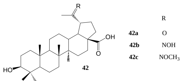
Fig. 5. C-20 modified betulinic acid derivatives
