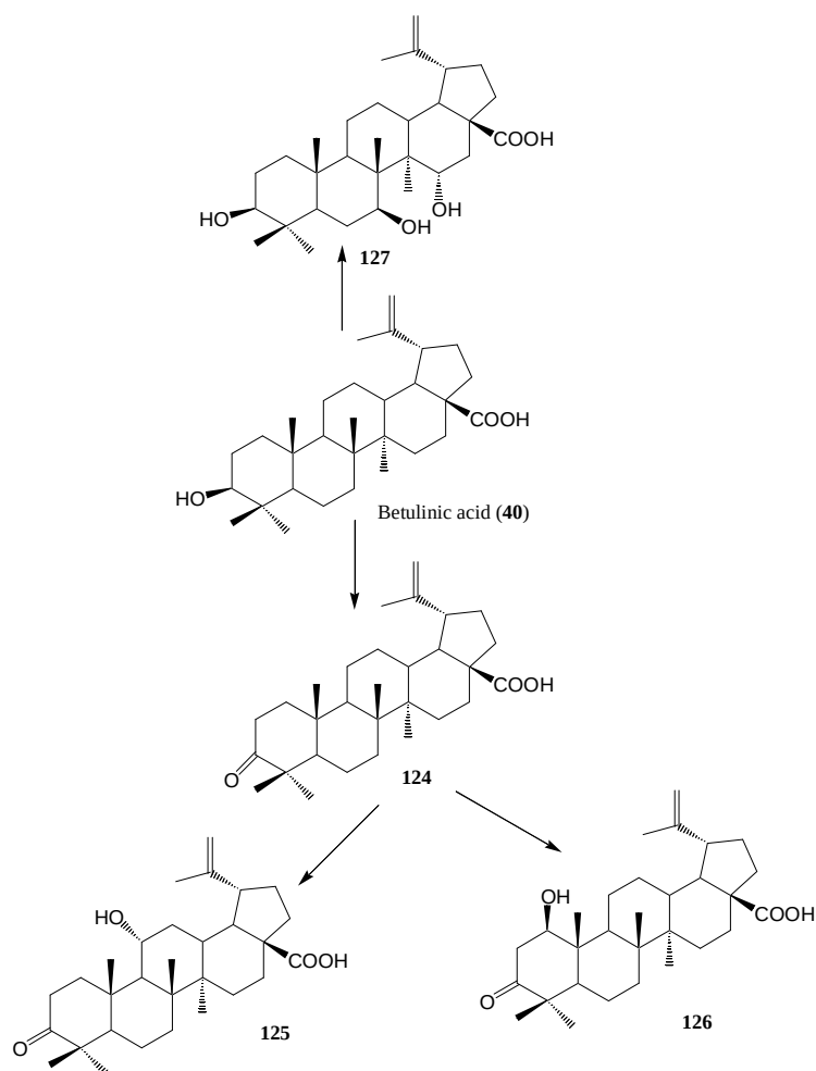
Fig.18. Proposed metabolic pathway for betulinic acid in Bacillus megaterium ATCC 13368
