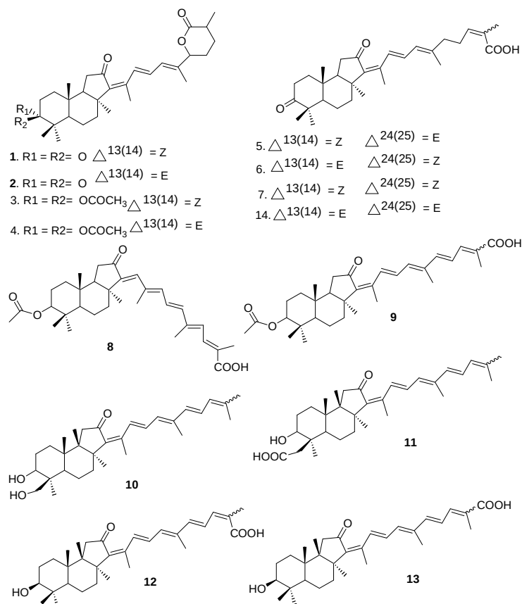
Fig.1. Isomalabaricane type triterpenoids stellettins from marine sponge.
