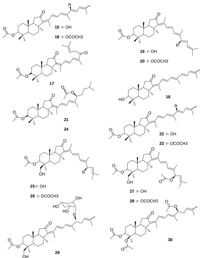
Fig. 2 Triterpenoid stelliferins from marine sponges
