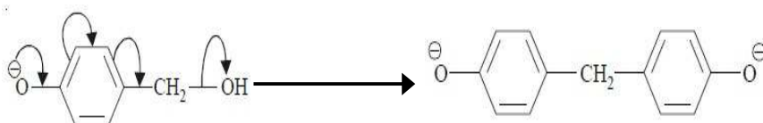
Fig. 4. Oxidation of phenol under alkaline conditions (Source: Mukherji, 2012)
