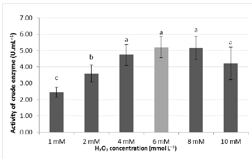
Fig. 2. Activity of crude peroxidase at different concentrations of hydrogen peroxide (pH 6.0)
