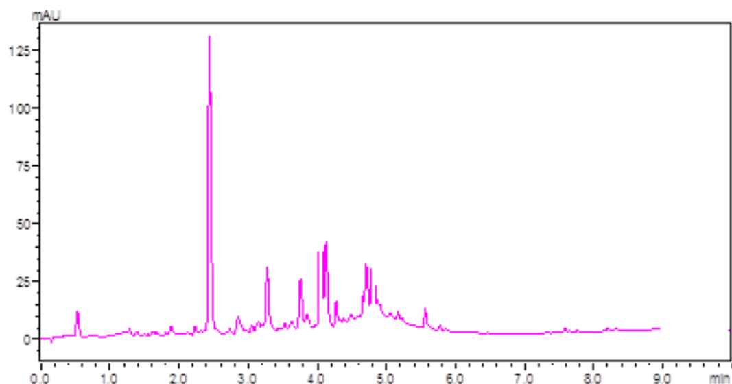
Figure 2: HPLC chromatograph for standard alliin elution
