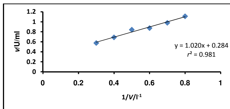
Fig. 1 Determination of the regression coefficient (slope) for the calculation of the minimum volume ( V_{\min} ) of substrate solution at maximum velocity, V_{\max} , of hydrolysis of substrate. V is volume of solvent in which the same mass of substrate is mixed to give any desired concentration. V_{\min} = 0.454 \pm 0.016 l; I_m = 5.3142 \pm 0.06 \exp(-8) \text{ m} ; Maximum [S]/([S]_{\max}) = 22.04 \pm 0.04 \text{ g/l}
