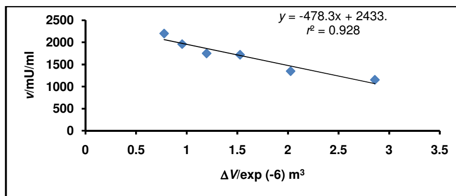
Fig. 3 The regression of v on excess volume ( \Delta V ) for the determination of translational entropy (TE) according to Eqs. 17, 18 and 19.
