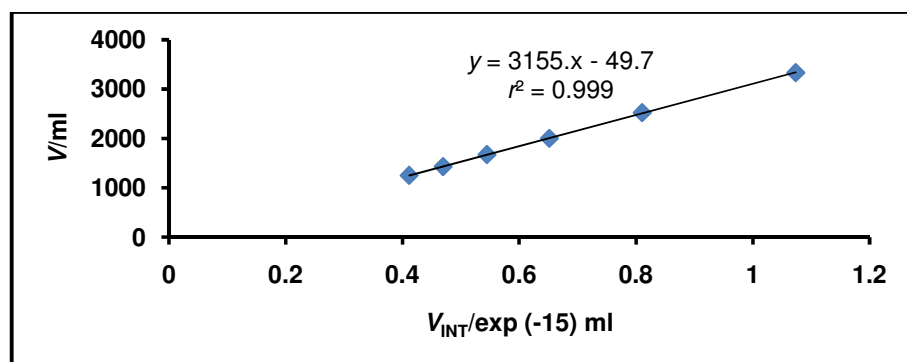
Fig. 2 The regression of volume ( V ) of the substrate solution on average interparticle volume ( V_{\text{INT}} ) for the determination of volume ( V_{\infty} ) at infinite dilution of the substrate concentration. V is volume of solvent in which the same mass of substrate is mixed to give any desired concentration; Total reaction mixture volume = 2ml. As shown in Eq. (12), I_{\infty} = 7.03 \pm 0.04 \exp(-7) \text{ m} ; V_{\infty} = 1.103 \pm 0.199 \exp(6) \text{ ml} . Prepared [S] for assay ranges from 3 g/l – 8 g/l \equiv 10 \text{ g}/3.333 \text{ l} - 10 \text{ g}/1.25 \text{ l} (see Table 1 for detail); the concentration [S]_{\infty \text{ dil}} at “infinite dilution” 9.215 \pm 1.659 \exp(-3) \text{ g/l} \equiv 10 \text{ g}/1103.49 \text{ l} .
