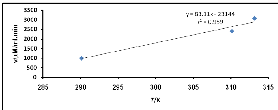
365 Fig. 3 Plot of velocity of hydrolysis of gelatinized starch versus absolute temperature ranging 366 from 290.15-313.15K for the determination changes in the radius of the 1:100 diluted, CaCl 2 367 treated crude HSαA showing increasing activity.
