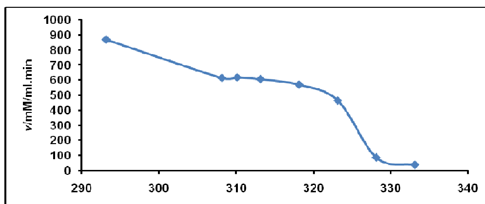
Fig. 1 A plot showing the trend of velocity (v) of hydrolysis of gelatinized potato starch with absolute temperature without additional calcium chloride (5mM/l) using 1:1000 diluted crude HS \alpha A.
