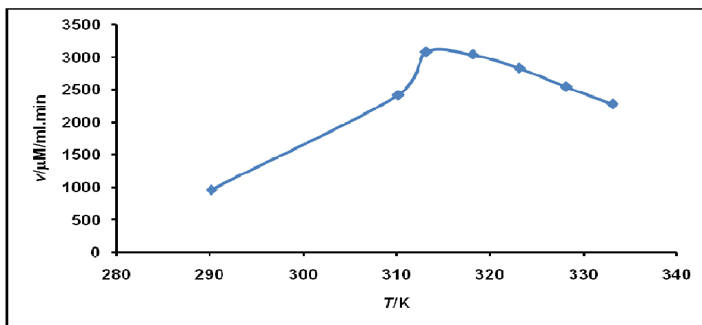
361 Fig. 2 A plot showing the trend of velocity of hydrolysis of gelatinized potato starch with 362 absolute temperature with additional calcium chloride (5mM/l) using 1:100 diluted crude HSαA.
