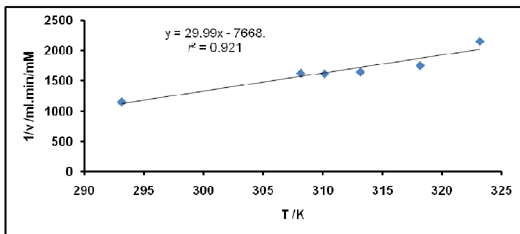
378 Fig. 5 A plot of the reciprocal of the velocity of hydrolysis of gelatinized potato starch without 379 calcium chloride versus temperature for the determination of changes in the radius of 1:1000 380 diluted HS \alpha A.
