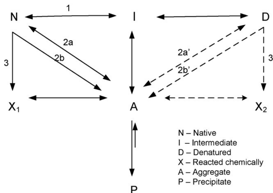
Figure no 1. Graphic illustration of protein aggregation
