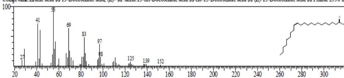
Figure 2g: GC-MS Fragment of Erucic acid
