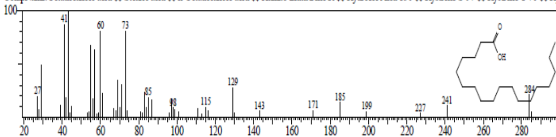
Figure 2c: GC-MS Fragment of Stearic acid
