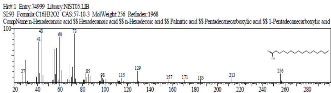
Figure 2b: GC-MS Fragment of Palmitic acid
