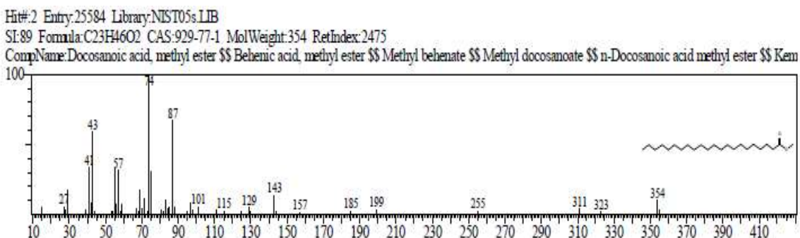
Figure 2i: GC-MS Fragment of Behenic acid
