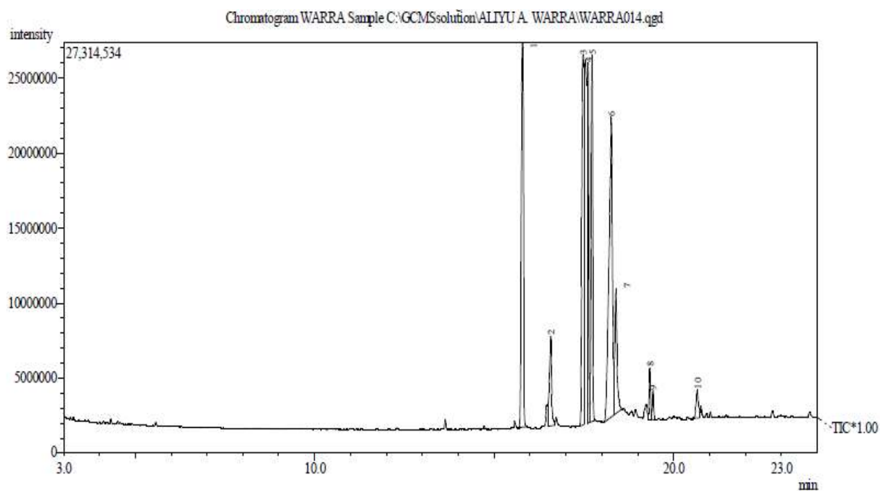
Figure 2a. Typical GC-MS total ionic chromatogram (TIC) of hexane extract of calabash seed oil.
