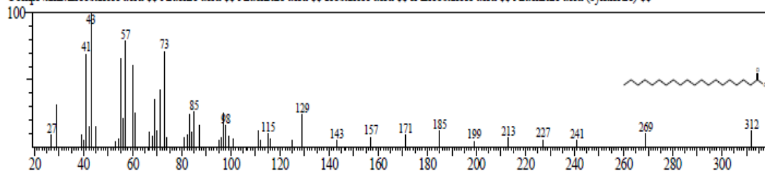
Figure 2h: GC-MS Fragment of Arachidic acid
