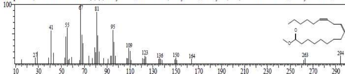
Figure 2e: GC-MS Fragment of Linoleic acid
