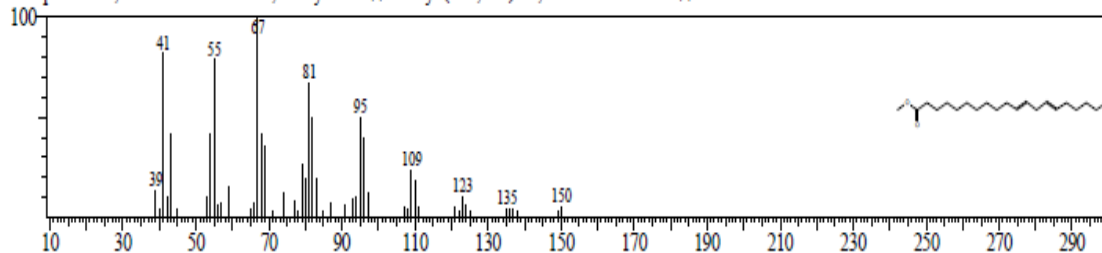
Figure 2d: GC-MS Fragment of Eicosadienoic acid
