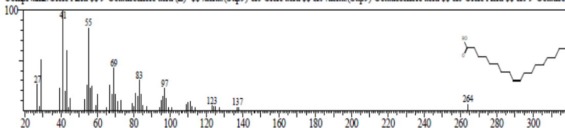
Figure 2f: GC-MS Fragment of Oleic acid
