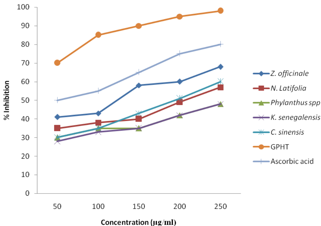
Figure 2: Comparative Hydroxyl radical scavenging activity of Zingiber officinale , Nauclea latifolia , Phyllanthus spp , Khaya senegalensis , Camellia Sinensis , GPHT and Ascorbic Acid. GPHT= Gingered Poly-Herbal Tea
