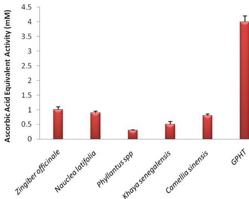
Figure 1: Comparative antioxidant activity of Zingiber officinale , Nauclea latifolia , Phyllanthus spp , Khaya senegalensis , Camellia Sinensis and GPHT. GPHT= Gingered Poly-Herbal Tea
