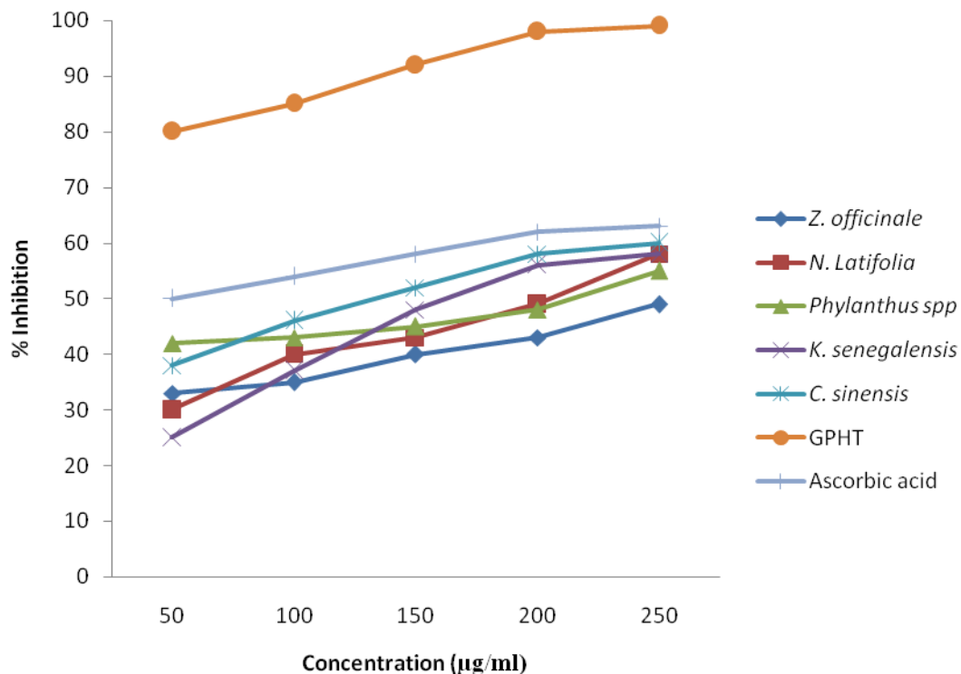
235 Figure 4: Comparative Superoxide radical scavenging activity of Zingiber officinale , 236 Nauclea latifolia Phyllanthus spp , Khaya senegalensis , Camellia Sinensis 237 GPHT and Ascorbic Acid. GPHT= Gingered Poly-Herbal Tea
