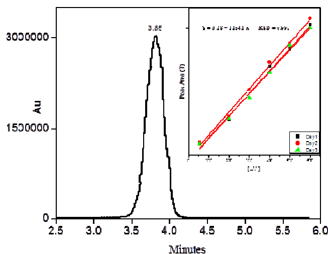
Figure 1. chromatogram of Vitamin C in serum samples. Inserted curve: The Calibration curve for the analysis of ascorbic acid standard samples.
