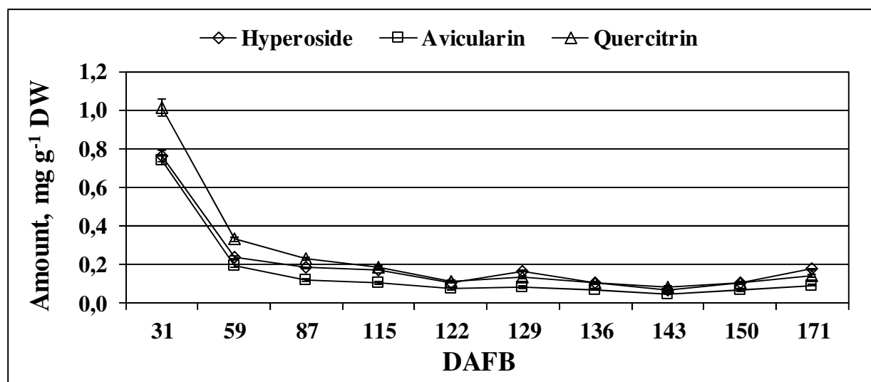
Fig. 2. Variation in the quantitative composition of quercitrin, hyperoside, and avicularin in apple samples throughout the vegetation period
