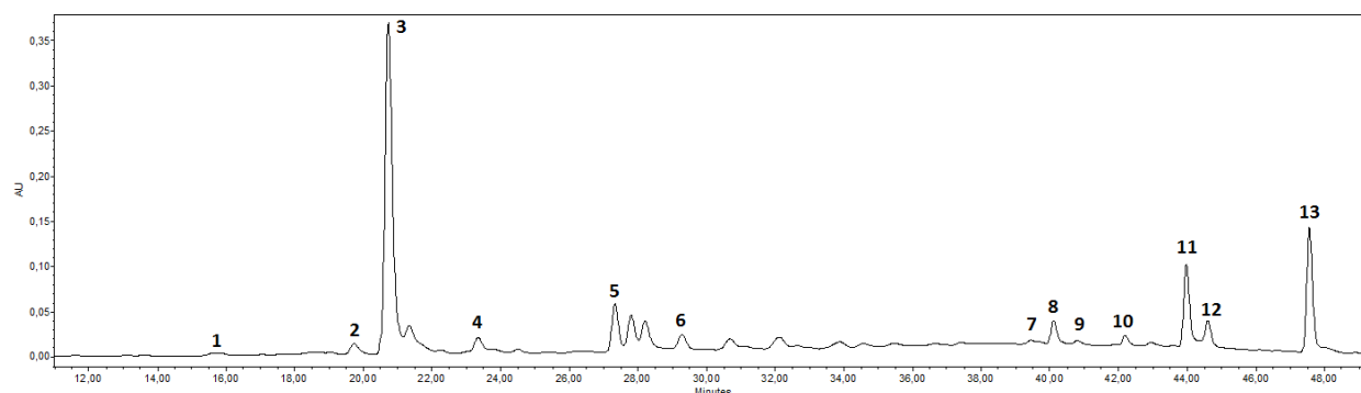
Fig. 1. Chromatogram of the ethanol extract of the 'Ligol' apple sample ( \lambda = 280 nm). Numbers indicate the peaks of analytes: 1: procyanidin B1, 2: (+)-catechin, 3: chlorogenic acid, 4: caffeic acid, 5: (–)-epicatechin, 6: rutin, 7: hyperoside, 8: isoquercitrin, 9: avicularin, 10: quercitrin, and 11: phloridzin.
