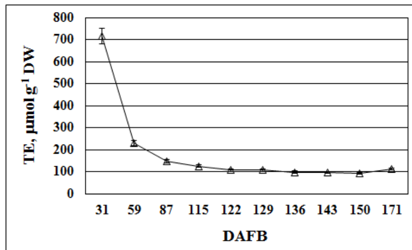
Fig. 8. Variation in the reduction activity of apple sample extracts throughout the vegetation period
