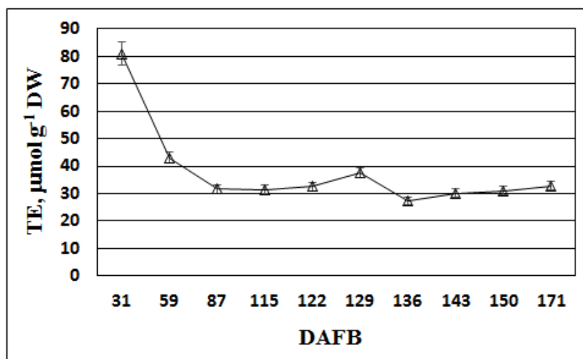
Fig. 7. Variation in the antiradical activity of apple sample extracts throughout the vegetation period
