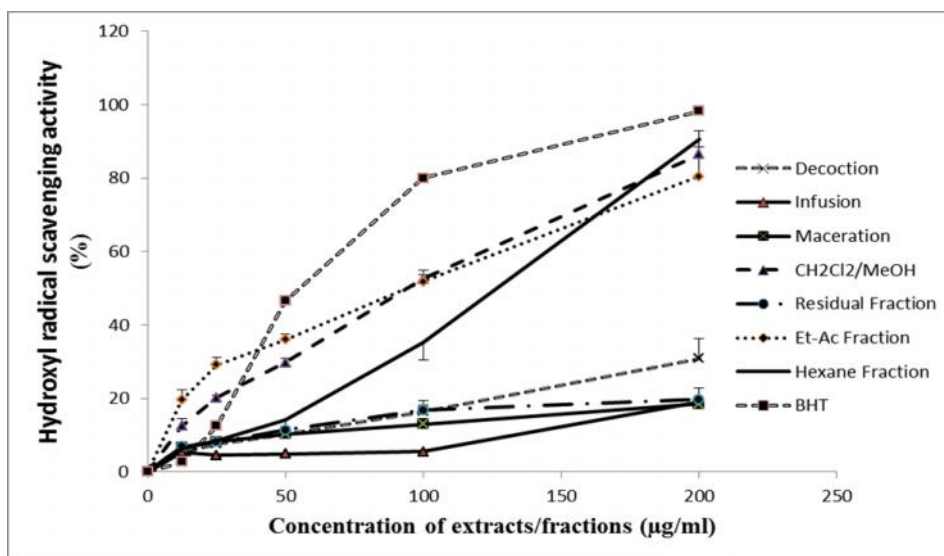
Figure 1: Hydroxyl radical scavenging activities of extracts/fractions of Curcuma longa L.
