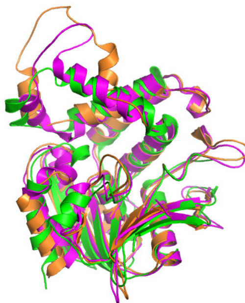
Fig. 11. Ribbon diagram showing superimposition of SaHTA (green), HtHTA (magenta) and LtHTA (orange), with the nearly identical \alpha/\beta core structures but with differences in the size and orientation of the surface loops.
