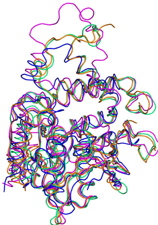
Fig. 7. Ribbon diagram showing the superimposition of DcsE (Orange), H HTA (green), L HTA (magenta) and SaHTA (blue). (Figure was generated by using VMD program [79]).
