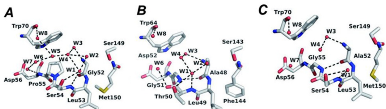
422 423 Fig. 8. Changes in the orientation of the \beta turn in the active site of (A) native DcsE, (B) H HTA and (C) 424 G52A/P55G mutant of DcsE. (Figure from Oda, et al. [78]). 425
