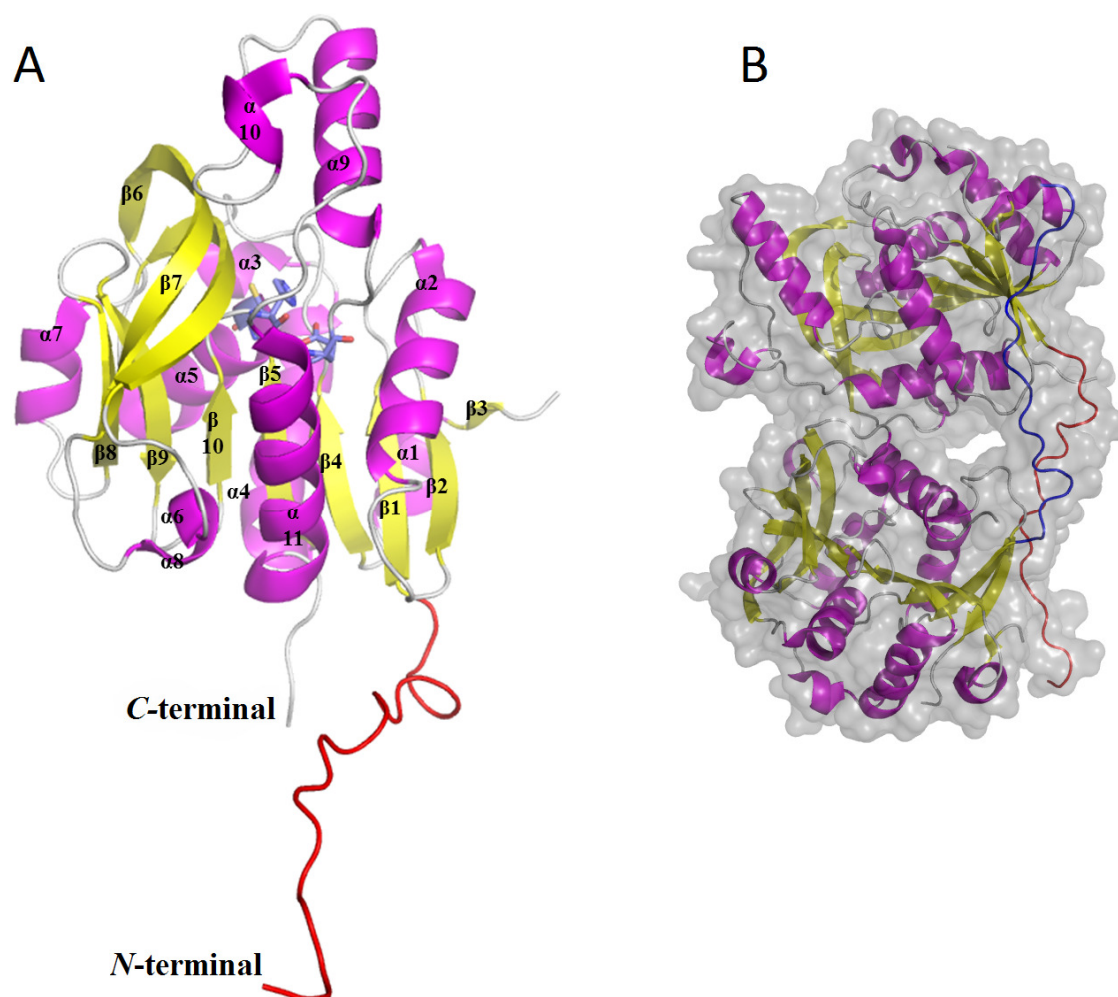
Fig. 12. (A) Structure of the BcHTS subunit organized into a single domain. Alpha helices are colored in magenta, beta sheets are yellow and the N -terminal region is shown in red. The catalytic triad constituting Cys, His and Glu are shown by blue sticks. (B) Quaternary structure of BcHTS showing N -terminal beta-strand exchange between the monomers. The N -terminal region of one monomer is colored red and the other is blue.
