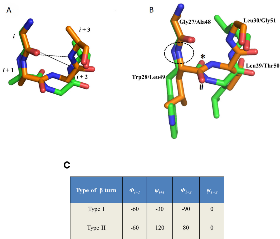
311 Fig. 5. (A) Idealized type-I \beta -turn (orange) overlaid on an idealized type-II \beta -turn (green). The amino acids 312 are XxxAlaAlaXxx, where Xxx indicates an incompletely specified residue. C \alpha of each residue is labeled; 313 dotted lines indicate hydrogen bonds between the carbonyl of residue i and the amide of residue i+3 . (B) 314 Superimposed structures of the oxyanion loop regions of PFE (green, a type-II \beta -turn) and H / H TA 315 (orange, a type-I \beta -turn). The carbonyl of Trp28 in PFE (*) points toward the active site, whereas for 316 H / H TA the carbonyl of Leu49 (#) points away from the active site. In both cases the backbone amide of 317 residue i+1 (dashed circle) points toward the active site because it forms a hydrogen bond with the 318 oxyanion intermediate. (C) Table showing the ideal angles for different types of beta-turns (Figure derived 319 from Jiang, et al. [64]).
