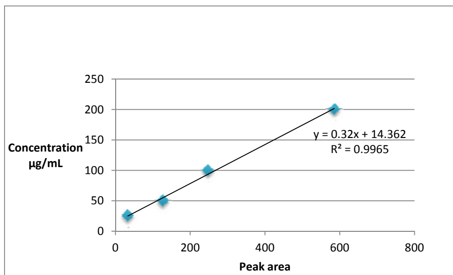
Figure 3: Oxytetracycline calibration curve.
