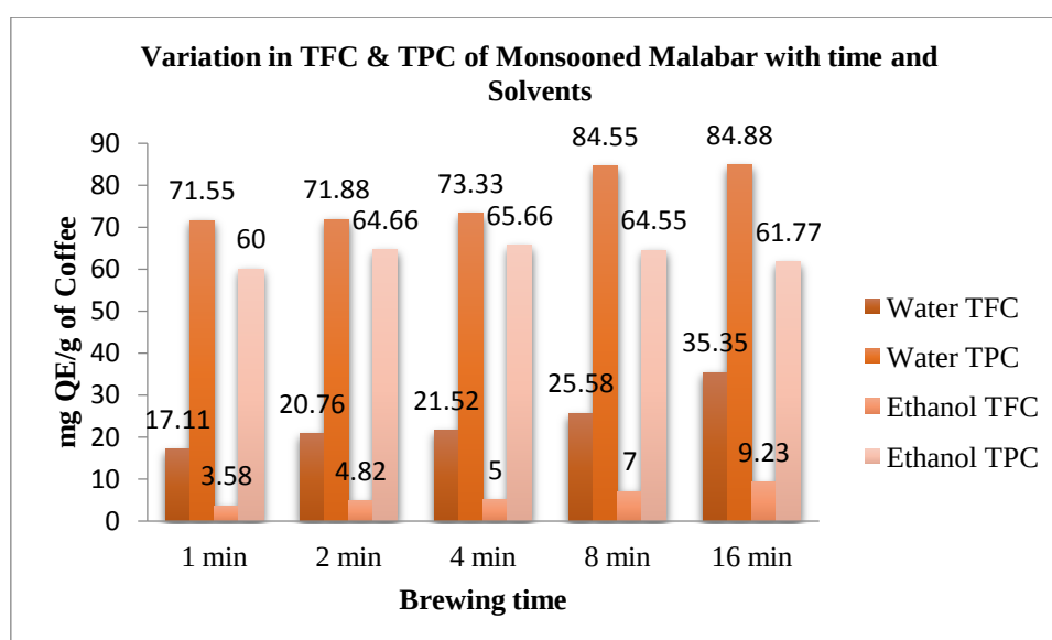
Figure 13: Total Flavonoid and Phenolic Content variation in roasted coffee Monsooned Malabar with time and solvents.
