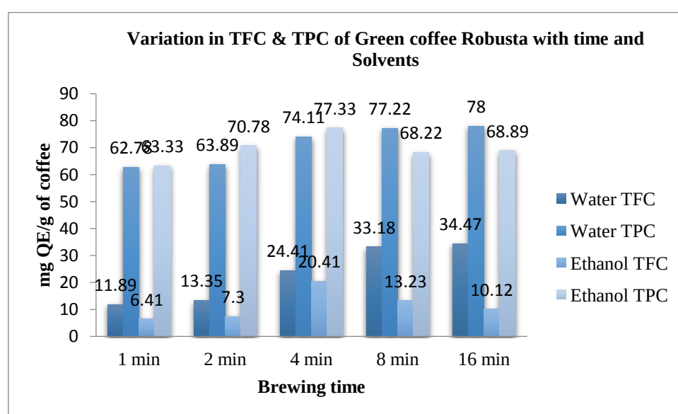
428 Figure 14: Total Flavonoid and Phenolic Content variation in green coffee Coffea robusta with time and 429 solvents.
