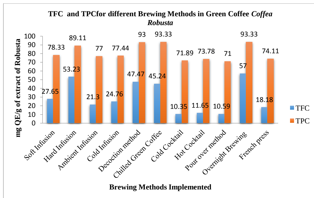
Figure 04: Total Flavonoid and Phenolic Content in various Brewing Methods followed for Coffea Robusta
