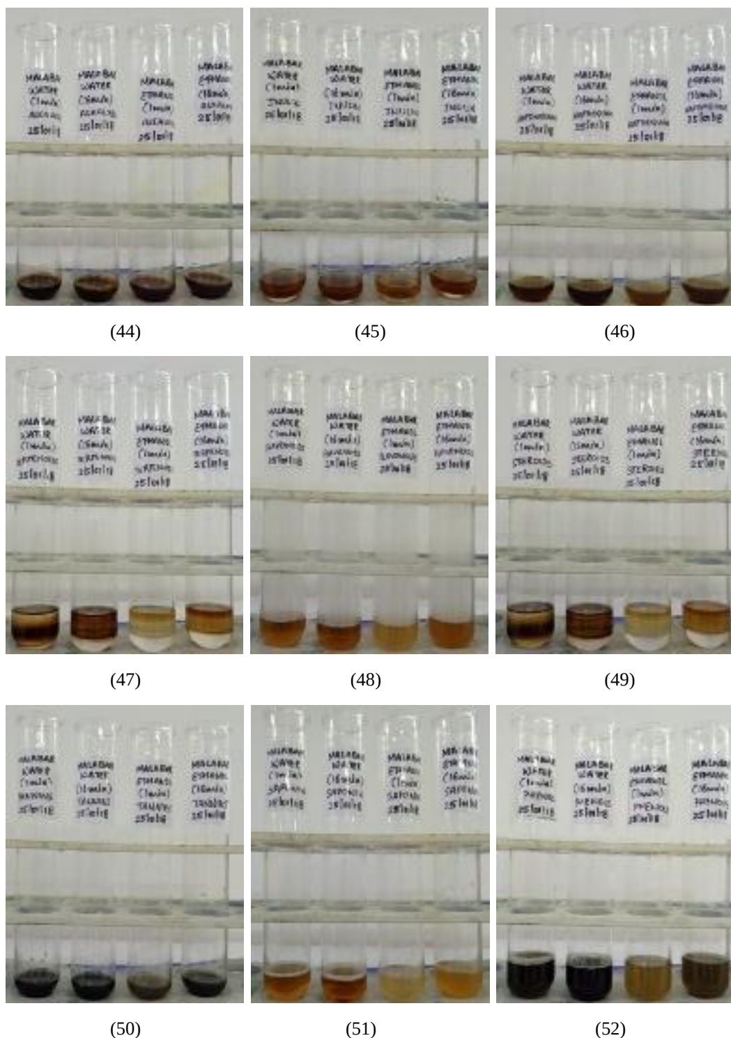
Figure 10: (44-52) Phytochemical screening for the presence of secondary metabolites of roasted coffee Malabar for 1 min and 16 min in Ethanol and distilled water.
