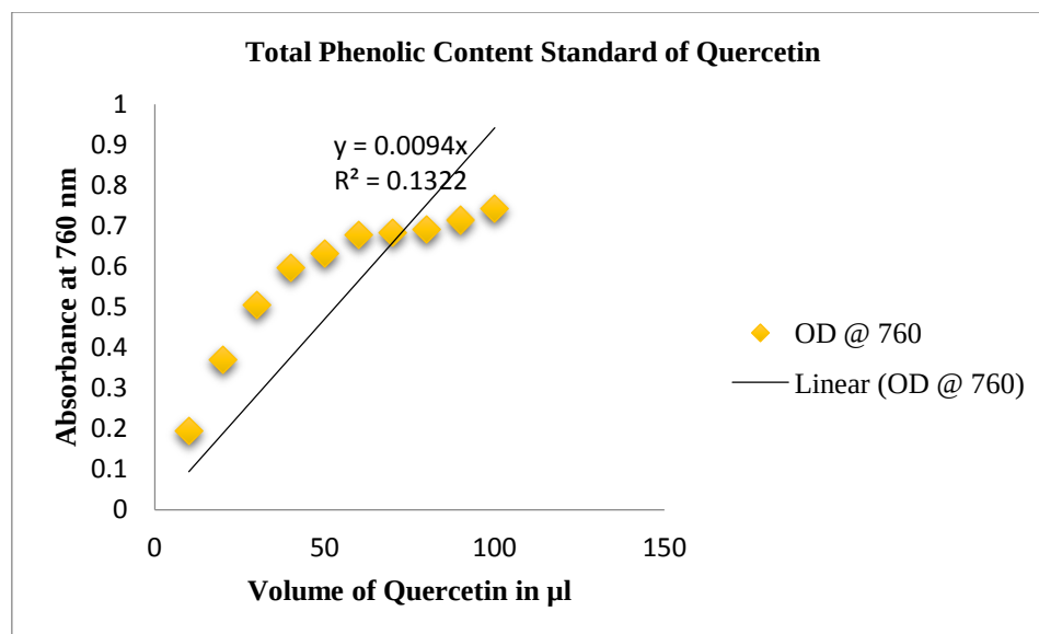
Figure 12: Standard for Total Phenolic Content.
