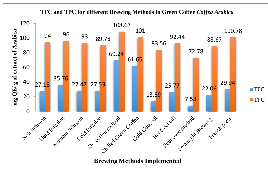
Figure 02: Total Flavonoid and Phenolic Content in various Brewing Methods followed for Coffea Arabica
