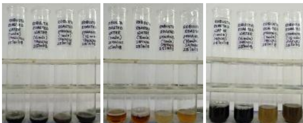
Figure 09: (35-43) Phytochemical screening for the presence of secondary metabolites of roasted coffee Coffea robusta for 1 min and 16 min in Ethanol and distilled water.
