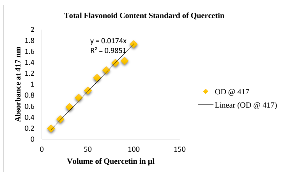
Figure 11: Standard for Total Flavonoid Content.
