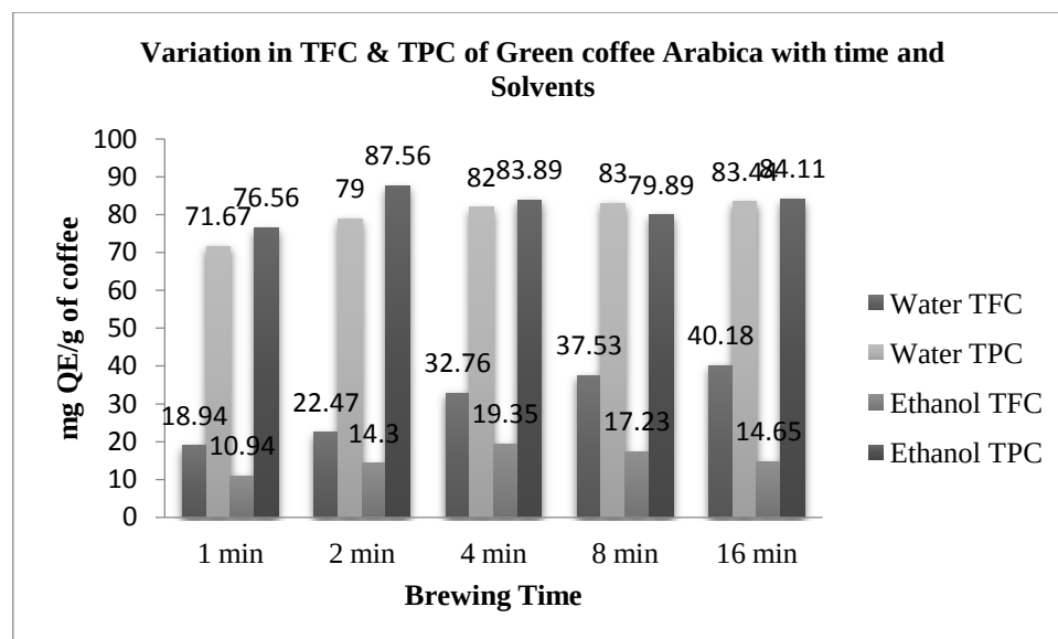
Figure 15: Total Flavonoid and Phenolic Content variation in green coffee Coffea arabica with time and solvents.
