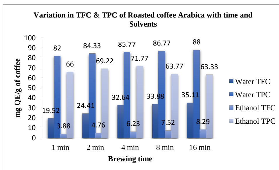
Figure 17: Total Flavonoid and Phenolic Content variation in roasted coffee Coffea arabica with time and solvents.
