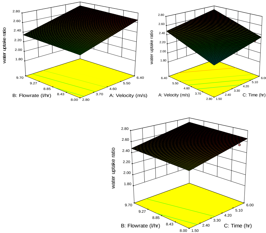
Fig 2: Variation of water uptake ratio with velocity, flow rate and humidification time
