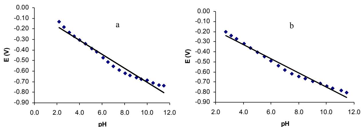
Figure 2. Dependence of cathodic peak potentials as a function of pH for Sudan I a) SWV ( 7.41 \times 10^{-6} M), in B-R (0.04 M) buffer, v = 200 mV/s, b) DPP ( 1.96 \times 10^{-5} M) in 50% B-R (0.02 M) buffer-50% ethanol medium, v = 4 mV/s.
