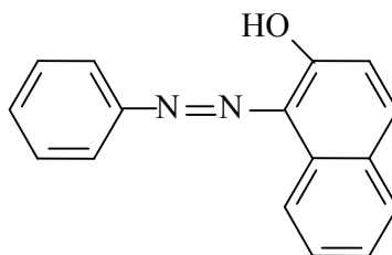
Scheme 1. Molecular structure of the Sudan I.
