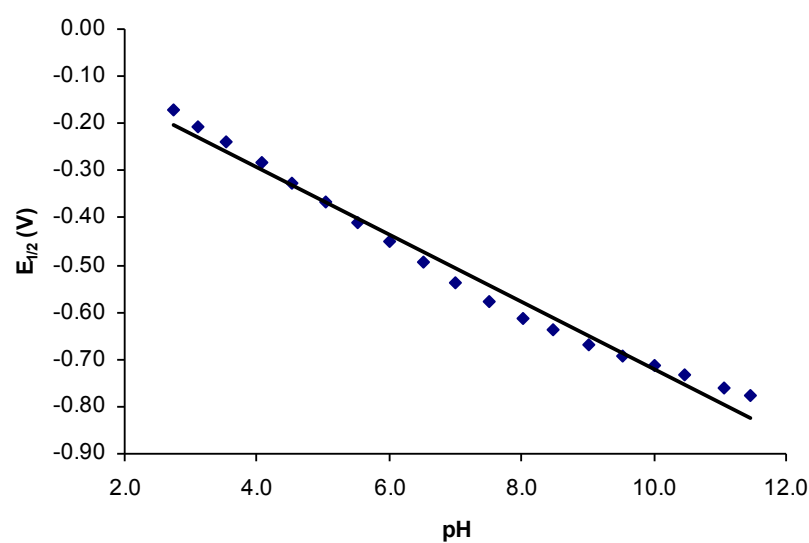
Figure 6. The dependence of E_{1/2} values of Sudan I on pH in 50% BR (0,02 M) buffer-50% ethanol medium, v = 4 mV/s.
