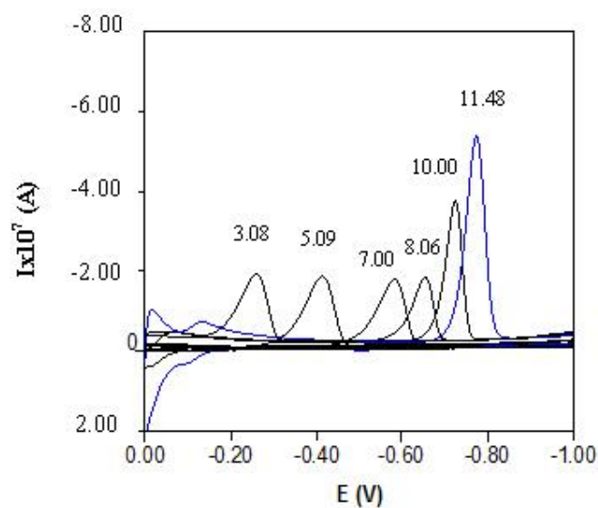
Figure 8. CV voltammograms of 7,41 \times 10^{-6} M Sudan I in B-R (0.04 M) buffer, (pH 3.08, 5.09, 7.00, 8.06, 10.00, and 11.48, \nu = 200 mV/s).
