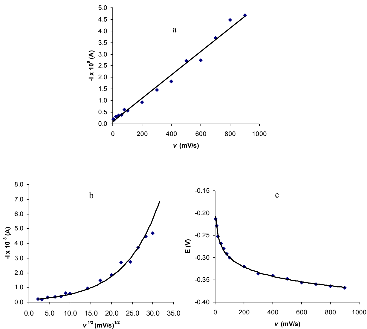
Figure 10. a) The change of cathodic peak currents of 9.90 \times 10^{-6} M Sudan I with scan rate at pH 4.15 in B-R (0.04 M) buffer b) The change of cathodic peak currents with square root of scan rate at pH 4.15, c) The change of cathodic peak potentials with scan rate at pH 4.15, \nu=5 -1000 mV/s.
