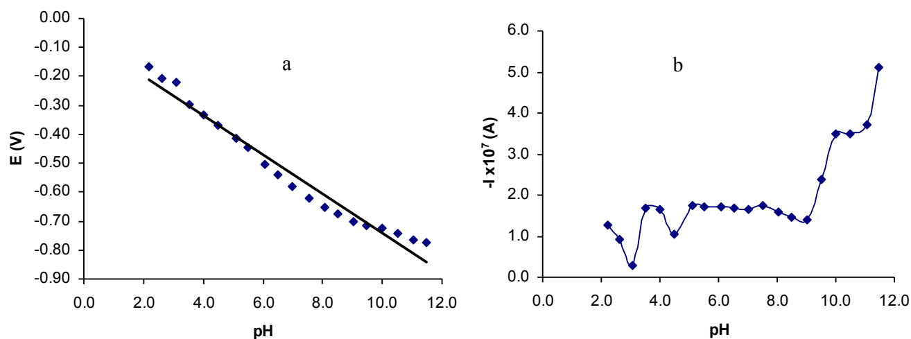
Figure 9. Dependence of a) cathodic peak potentials and b) cathodic peak currents as a function of pH in B-R (0.04 M) buffer obtained for 7.41 \times 10^{-6} M solution of Sudan I for CV technique.
