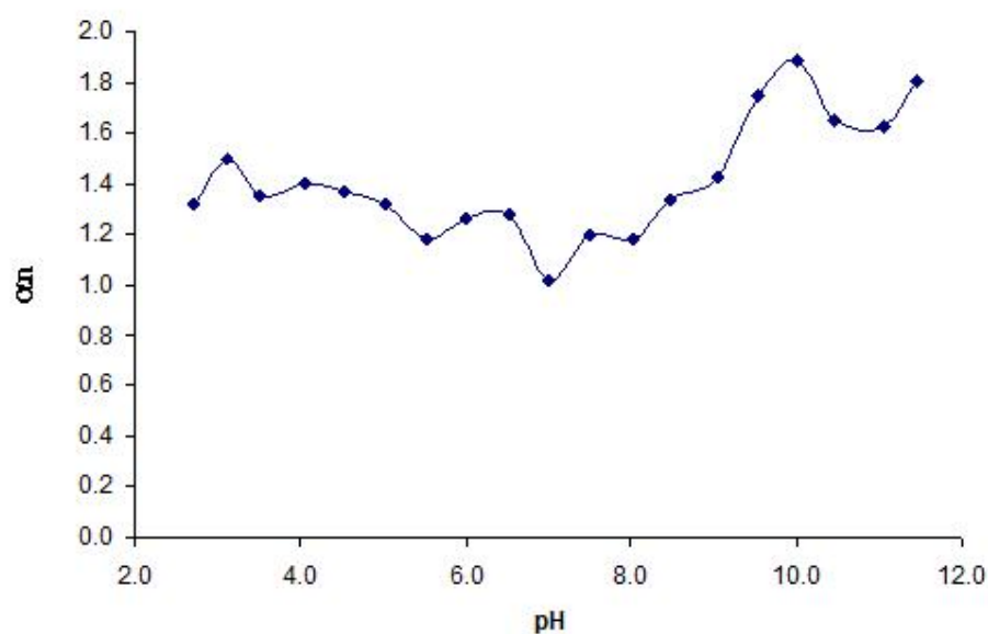
Figure 7. The change of \alpha n with pH for the Sudan I in 50% BR (0,02 M) buffer-50% ethanol medium.
