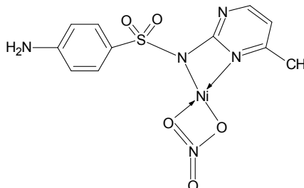
Fig. 2 (b) [Ni(SM)(NO 3 )]
