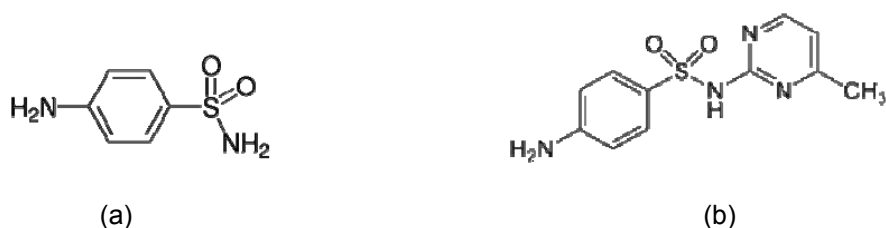
Fig. 1. Chemical Structure of Sulfadugs (a) Sulfanilamide and (b) Sulfamerazine.
