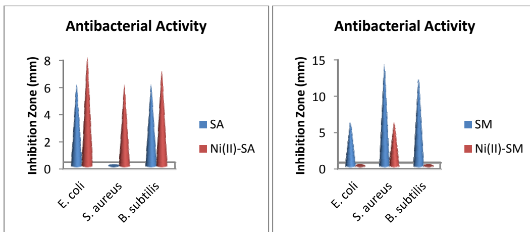
Fig.11. Comparative study of biological activity shown by drugs and their Nickel(II) complexes.
