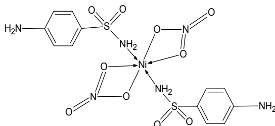
Fig. 2 (a) [Ni(SA) 2 (NO 3 ) 2 ]
