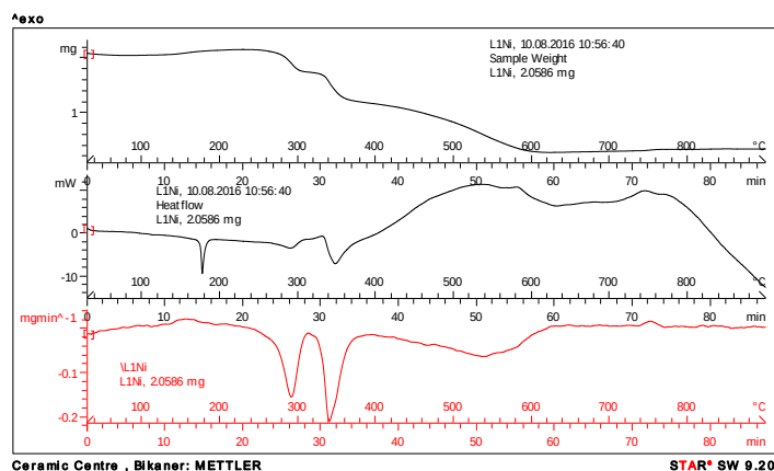
Fig. 6. Thermogravimetric analysis (TGA), Differential thermogravimetric analysis (DTA) and Derivative thermogravimetric (DTG) curves for Ni(II)-Sulfanilamide complex.
