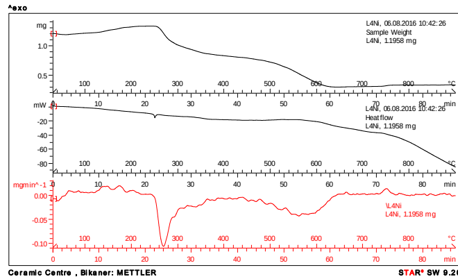
254 Fig. 7. Thermogravimetric analysis (TGA), Differential thermogravimetric analysis 255 (DTA) and Derivative thermogravimetric (DTG) curves for Ni(II)-Sulfamerazine 256 complex.
