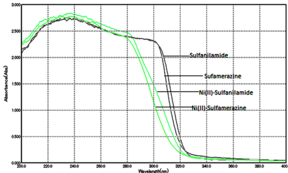
Fig. 3. UV-VIS Spectra of Ligands and their Nickel(II) Complexes.
