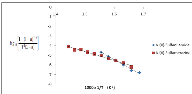
286 287 288 Fig. 8. Coats Redfern plot for second stage of decomposition for both the complexes . 289
