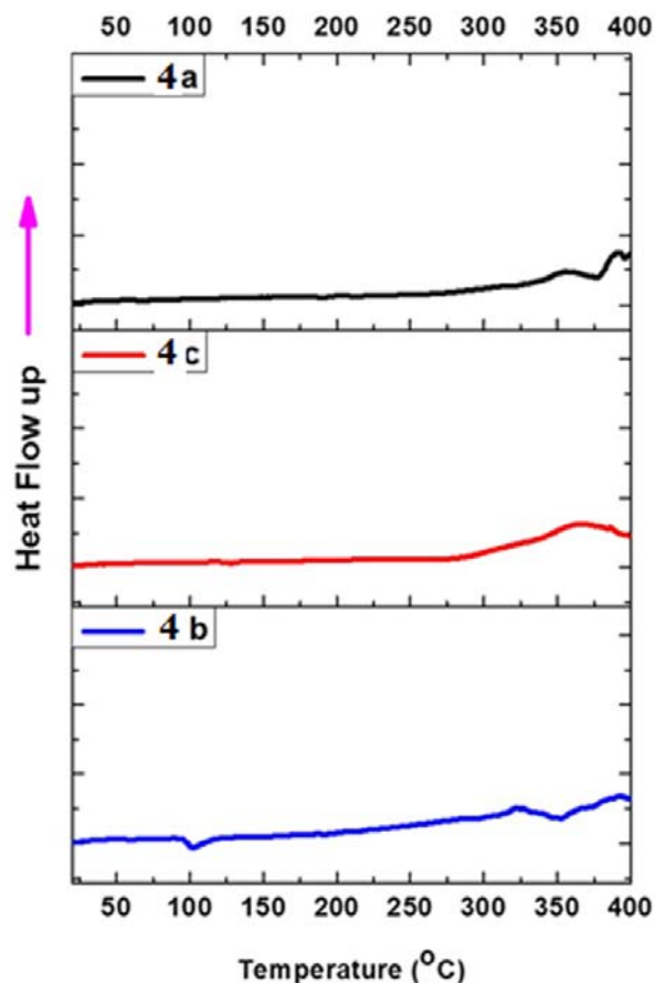
Figure 3. DTA of unsaturated terpolyesters 4a, 4b and 4c
