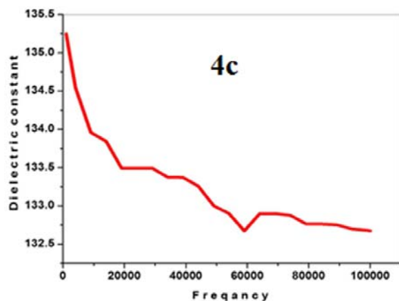
Figure 10. Relation between dielectric constant and frequency for terpolyester 4 c.
