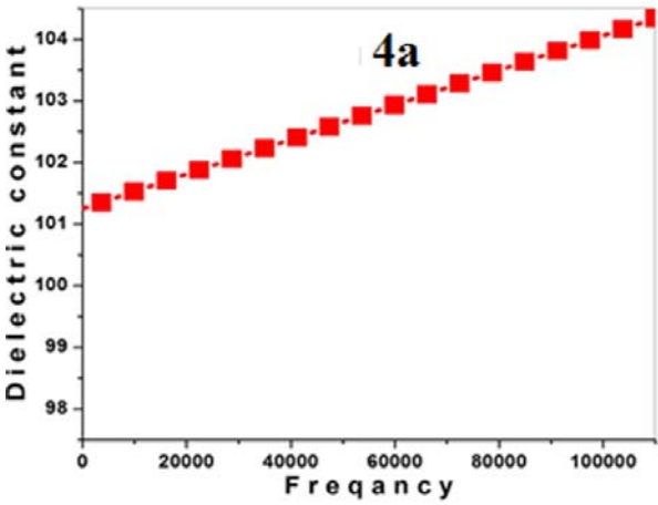
Figure 8. Relation between dielectric constant and frequency for terpolyester 4 a.
