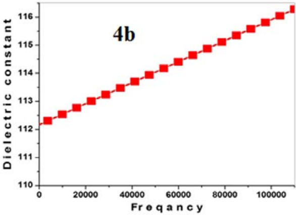
Figure 9. Relation between dielectric constant and frequency for terpolyester 4 b.
