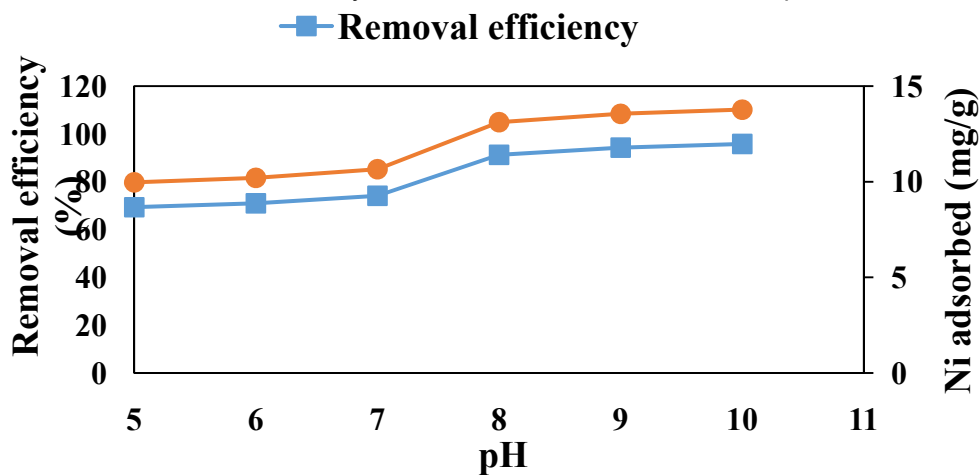
Fig. 3. Effect of pH on the adsorption of \text{Ni}^{2+} ions using the PG-M sorbent.
