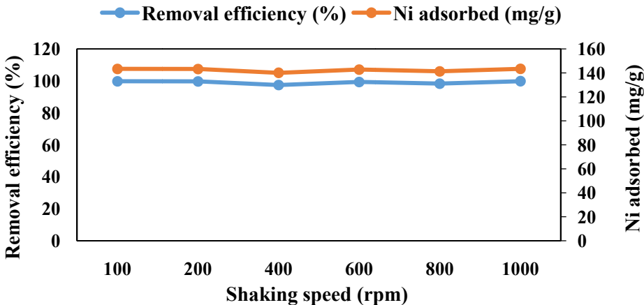
Fig. 5. Effect of shaking speed on the removal efficiency of \text{Ni}^{2+} ions using the PG-M sorbent.
