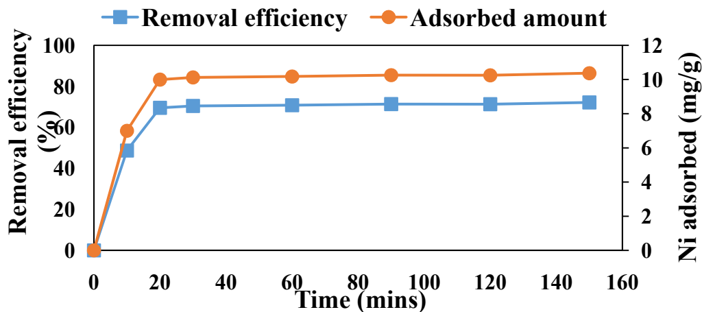
Fig. 2. Effect of contact time on the removal efficiency of \text{Ni}^{2+} ions using the PG-M sorbent.
