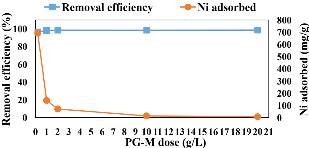
Fig. 4. Effect of the PG-M dose on the adsorption of \text{Ni}^{2+} ions.
