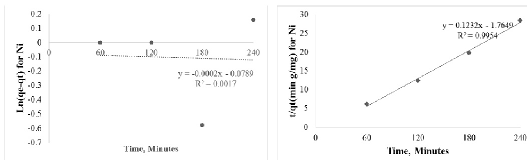
Figure 3: First and second order linearity test for \text{Pb}^{2+} (a), \text{Cu}^{2+} (b), \text{Cr}^{2+} (c) and \text{Ni}^{2+} (d) adsorption on M. oleifera
