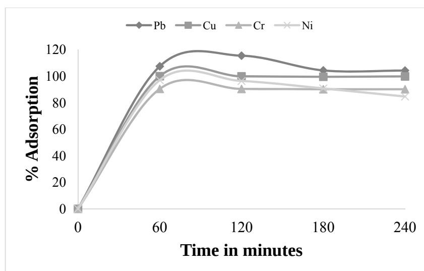
Figure 2: Effect of contact time on sorption of Pb^{2+} , Ni^{2+} , Cu^{2+} and Cr^{3+} ions by 5 g of M. oleifera
