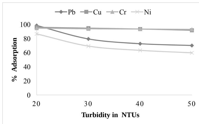
Figure 1: Effect of turbidity on percentage sorption of Pb^{2+} , Cu^{2+} , Cr^{2+} and Ni^{2+} ions onto M. oleifera
