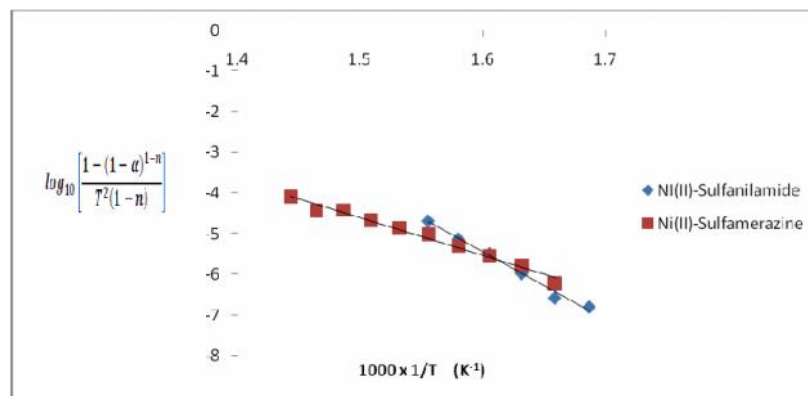
284 285 286 Fig. 8. Coats Redfern plot for second stage of decomposition for both the complexes . 287
