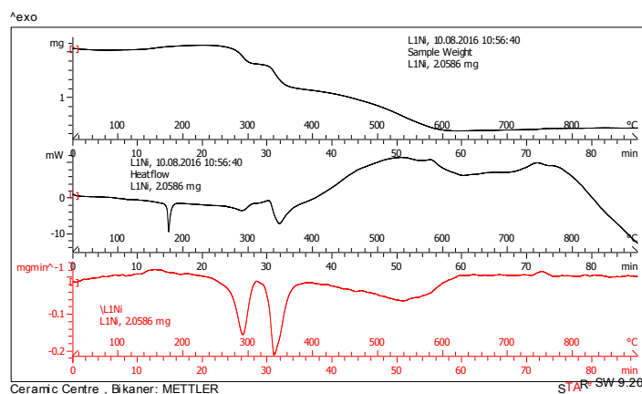
233 234 235 Fig. 6. Thermogravimetric analysis (TGA), Differential thermogravimetric analysis 236 (DTA) and Derivative thermogravimetric (DTG) curves for Ni(II)-Sulfanilamide complex.
