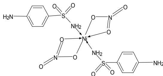
Fig. 2 (a) [\text{Ni}(\text{SA})_2(\text{NO}_3)_2]
