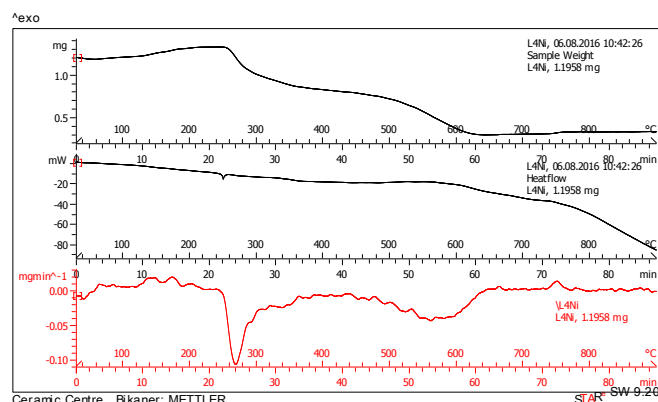
Fig. 7. Thermogravimetric analysis (TGA), Differential thermogravimetric analysis (DTA) and Derivative thermogravimetric (DTG) curves for Ni(II)-Sulfamerazine complex.
