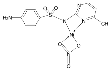
Fig. 2 (b) [\text{Ni}(\text{SM})(\text{NO}_3)]
