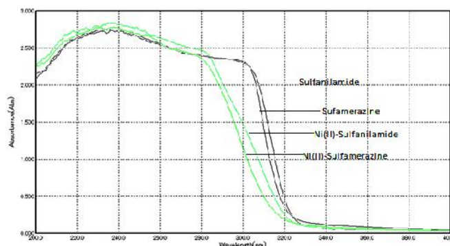
Fig. 3. UV-VIS Spectra of Ligands and their Nickel(II) Complexes.
