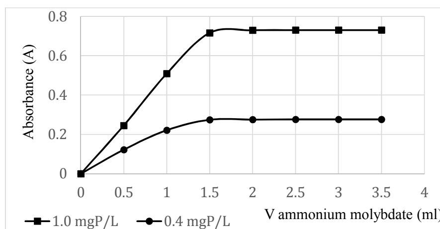
Figure 6. The effect of ammonium molybdate tetrahydrate in complex formation
