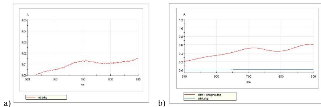
Figure 9. a) Absorbance spectrum of nitrite ions, b) The effect of nitrite ions in complex formation
