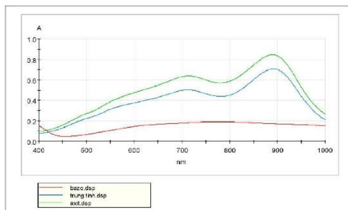
Figure 4. The role of base (red line), neutral (blue line) and acid (green line) environment in formation of phosphorus molybdate complex
