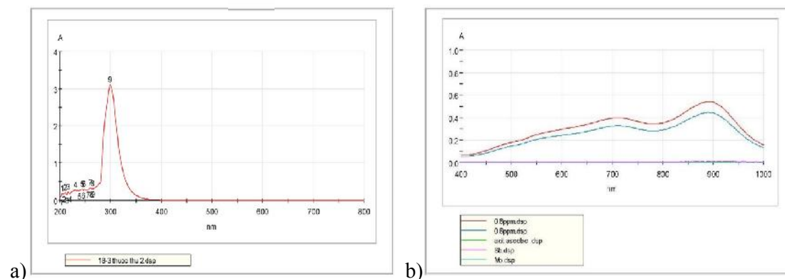
Figure 3. Absorption spectrum of color reagent (a), molybdenum blue phosphorus (b)
