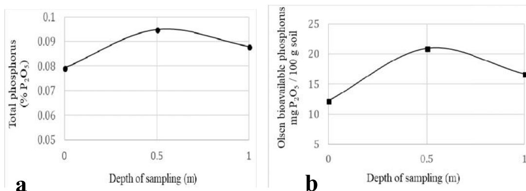
Figure 13. The effect of sampling location on a) total phosphorus, b) bioavailable phosphorus concentrations
