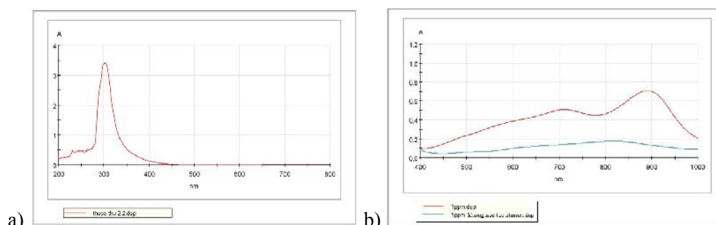
Figure 5. a) Absorbance spectrum of only potassium antimonyl tartrate, b) The role of potassium antimonyl tartrate hemihydrate in complex formation
