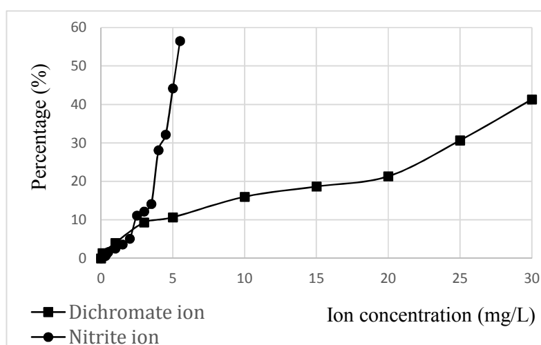
Figure 11. Effect level of nitrite and hexavalent chromium on phosphorus molybdate complex
