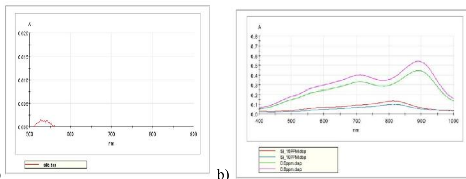
Figure 8. a) Absorbance spectrum of silicate ions, b) The effect of silicate ions in complex formation
