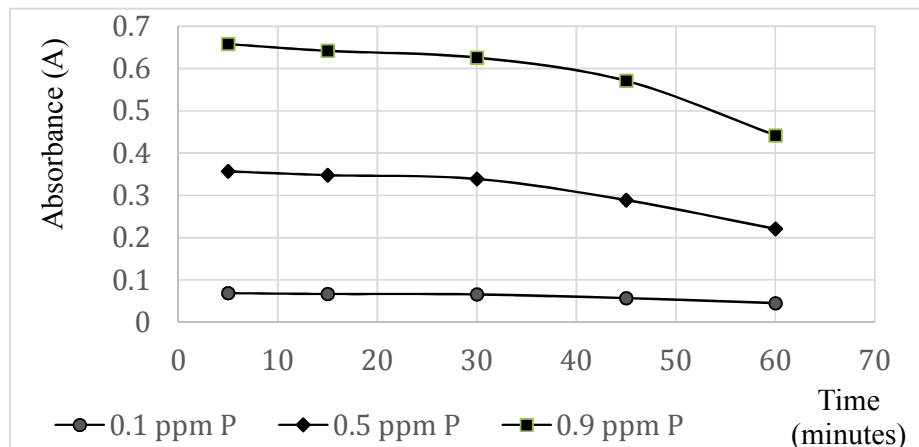
Figure 7. The stability of phosphorus molybdate complex
