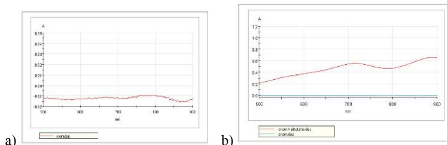
Figure 9. a) Absorbance spectrum of nitrite ions, b) The effect of nitrite ions in complex formation
