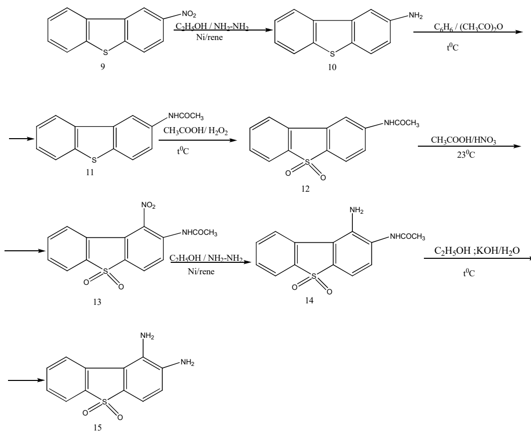
Scheme2. Synthesis of 1,2-diaminodibenzothiophene-5,5-dioxide
