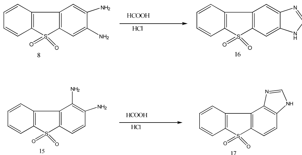
Scheme 3. Synthesis of 3H-imidazo[4,5-b]dibenzothiophene-5,5-dioxide (16) and 3H-imidazo[4,5-a]dibenzothiophene-5,5-dioxide (17).
