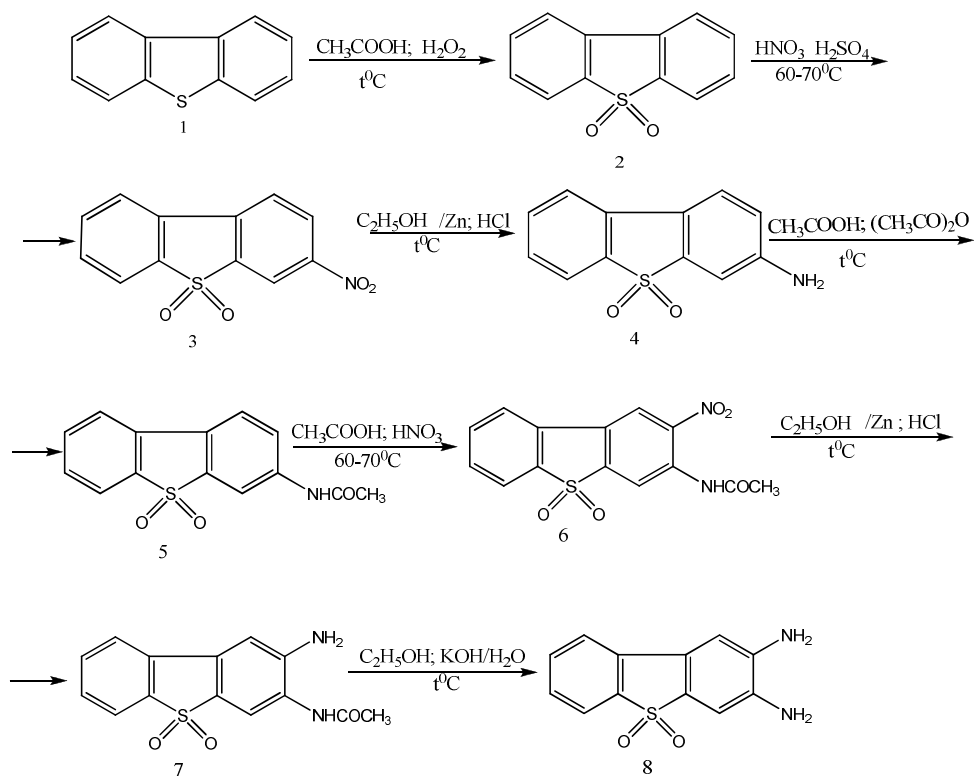
Scheme 1. Synthesis of 2,3 Diaminodibenzthiophene-5,5-dioxide
