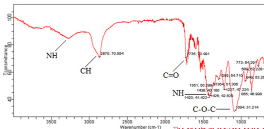
Fig. 1: IR spectrum of synthesized PUR sample
