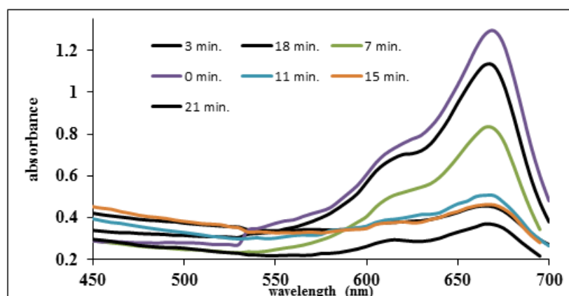
Fig. 4: UV-Vis spectra of MB during blank experiment in absence of PUR; MB= 4.6 \times 10^{-5} ; NaBH 4 =0.5M
