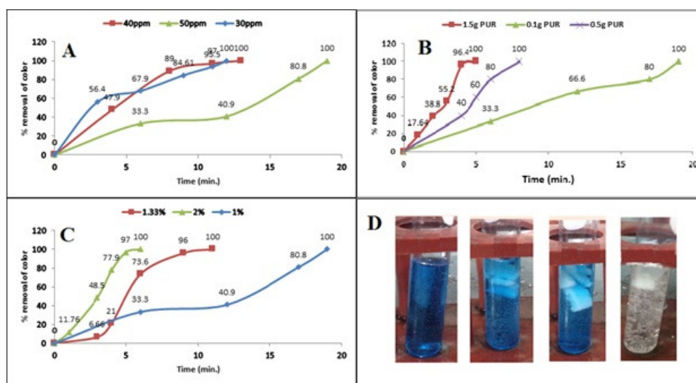
Fig. 5: Removal of dye (%) at different time intervals; A) 50ppm, 40ppm and 30ppm dye concentrations with 0.1g PUR and 1% \text{NaBH}_4 , B) 0.1g, 0.5g, 1.5g PUR with 1% \text{NaBH}_4 and 50ppm dye solution, C) 1%, 2% and 1.33% \text{NaBH}_4 with 50ppm dye solution and 0.1g PUR, D) progressive decrease in color of dye recorded by digital camera images
