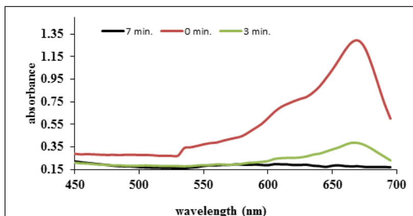
Fig. 3: UV-Vis spectra of MB during catalyzed reduction reaction. MB= 4.6 \times 10^{-5} ; NaBH 4 =0.5M and PUR= 0.1g
