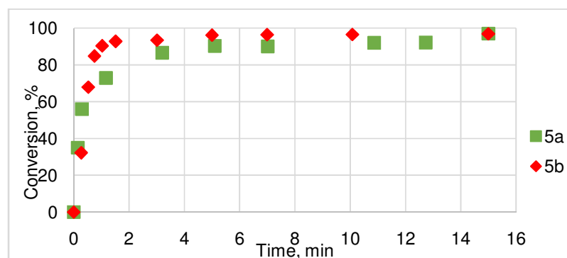
Fig. 2. Rates of condensation reactions of 4-methoxy- ( 5a ) and 2,4-dimethoxybenzaldehyde ( 5b ) with ethylcyanoacetate in IL ( 4d ) at 80 °C
