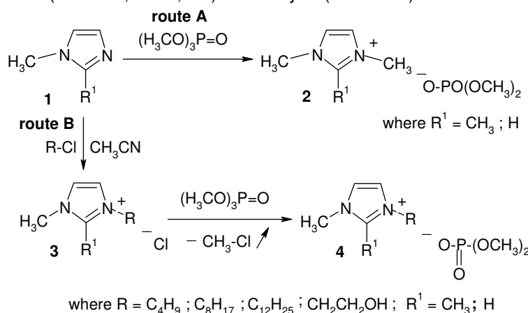
Scheme 1. Two routes to obtain imidazolium dimethyl phosphates (2, 4)
