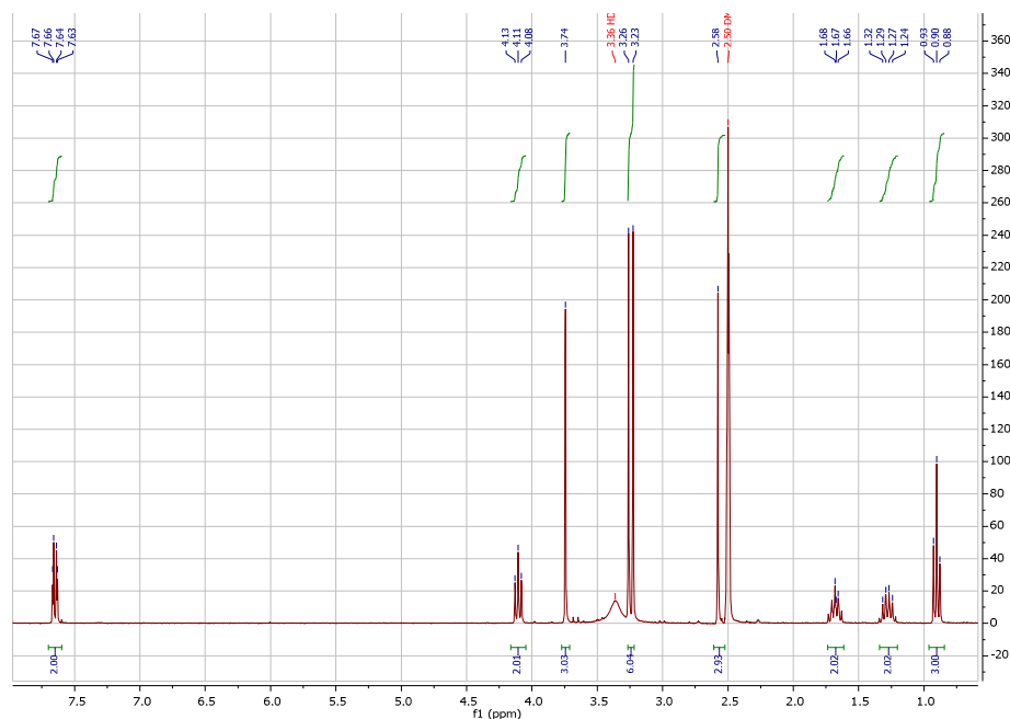
Fig. 1. 1 H NMR spectrum of 1-butyl-2,3-dimethylimidazolium dimethyl phosphate (4a)
