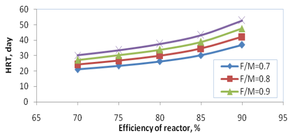
Fig. 7: Variation of HRT with efficiency of the anaerobic digestion
