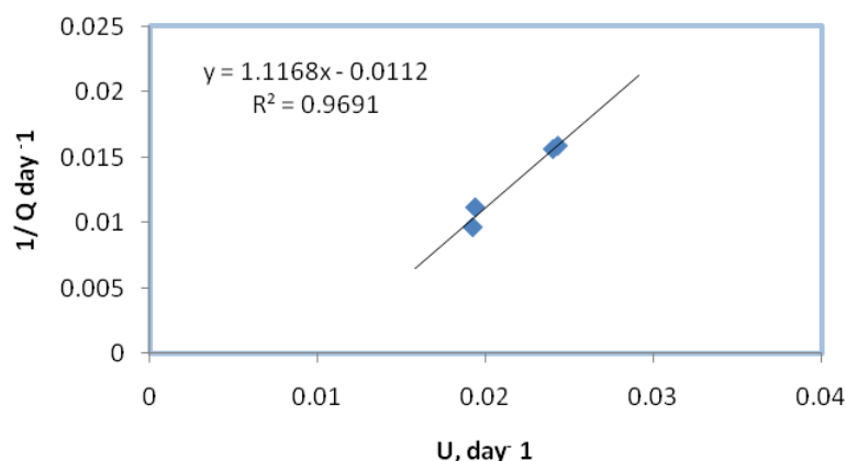
Fig. 6: Plot for determination of Y and K_d
