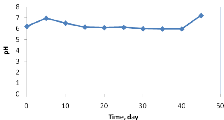
215 216 Fig 2. Effect of time on the pH
