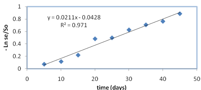
Fig. 4: First order kinetic plot
