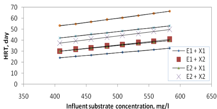
Fig. 9: Variation of HRT of the anaerobic reactor with influent substrate concentration ( E1=70\% , E2=80\% , E3=90\% , X1=510\text{mg/l} , X2=408\text{mg/l} )
