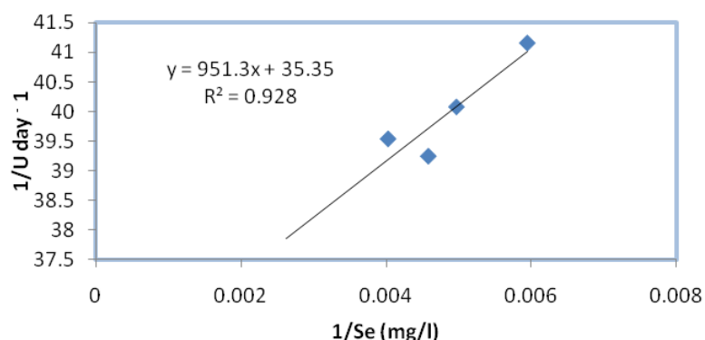
Fig. 5: Plot for determination of K and K_s
