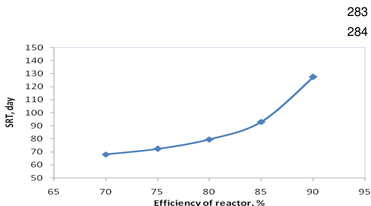
294 Fig. 8: Variation of SRT with efficiency of the anaerobic digestion
