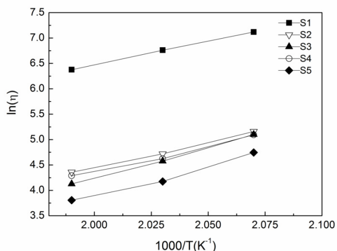
Fig 4. The plots of \ln(\eta) versus 1/T
