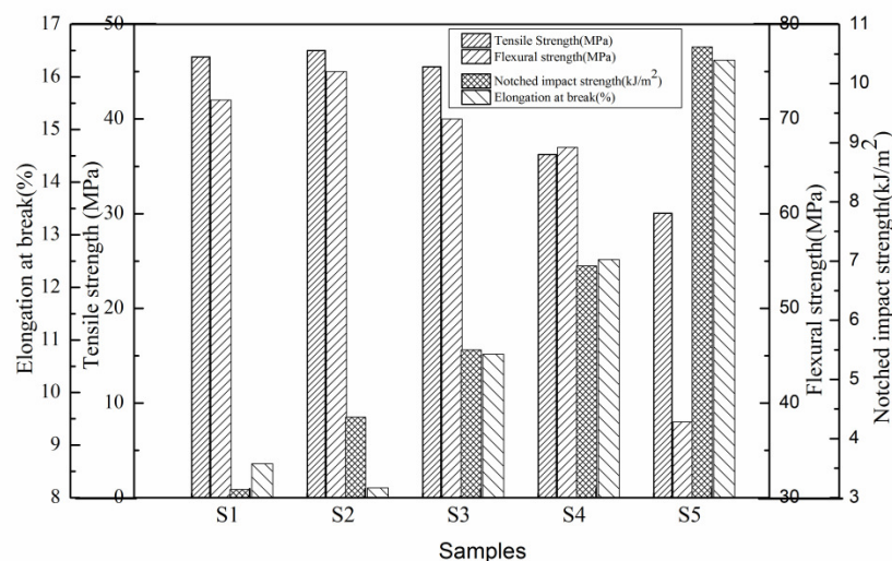
184 Fig 3. The values of tensile strength, flexural strength, izod impact strength and elongation at break.
