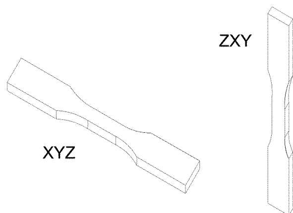
Fig 5. Specimens printed in the XYZ (horizontal) and ZXY (vertical) directions
