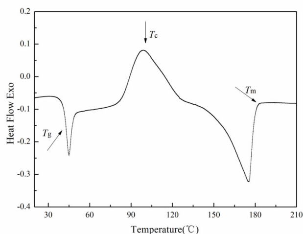
Fig 2. DSC thermograms of S3
