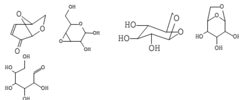
Levoglucosenone 3,4-Altrosan Levoglucosan 1,6-Anhydro-.beta.-d-talopyranose D-Allose (or Hexose)
