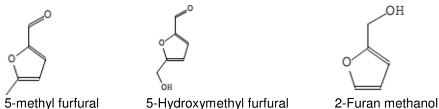
Figure 1: Structural formulae of furfural derivatives extracted from gmelina arborea leaves
