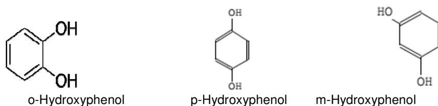
Figure 3: Structural formula of Hydroxyphenols extracted from gmelina arborea leaves.
