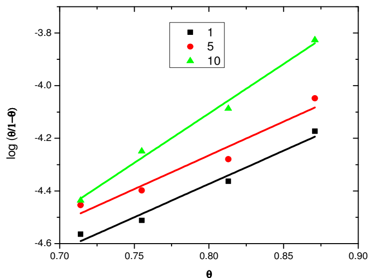
Fig. 8. Frumkin adsorption isotherm for inhibition of mild steel corrosion in 2.0 M HCl by different concentrations of 5-HTP at temperatures 303 K to 333 K [27].
