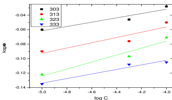
Fig. 6. Freundlich adsorption isotherm for inhibition of mild steel corrosion in 2.0 M HCl by different concentrations of 5-HTP at temperatures 303 K to 333 K [27].
