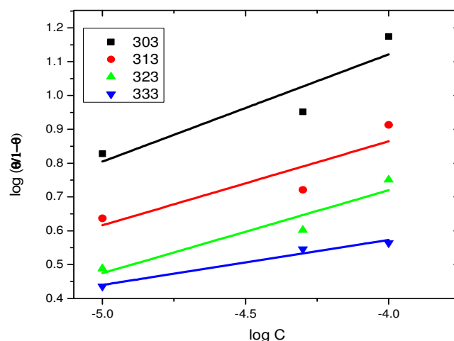
Fig. 9. El-Awady adsorption isotherm for inhibition of mild steel corrosion in 2.0 M HCl by different concentrations of 5-HTP at temperatures 303 K to 333 K [27].
