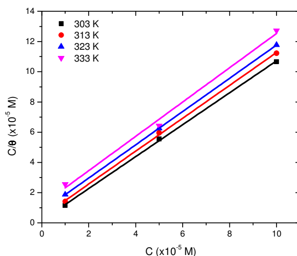
Fig. 4. Modified Langmuir adsorption isotherm for inhibition of mild steel corrosion in 2.0 M HCl by different concentrations of 5-HTP at temperatures 303 K to 333 K [27].
