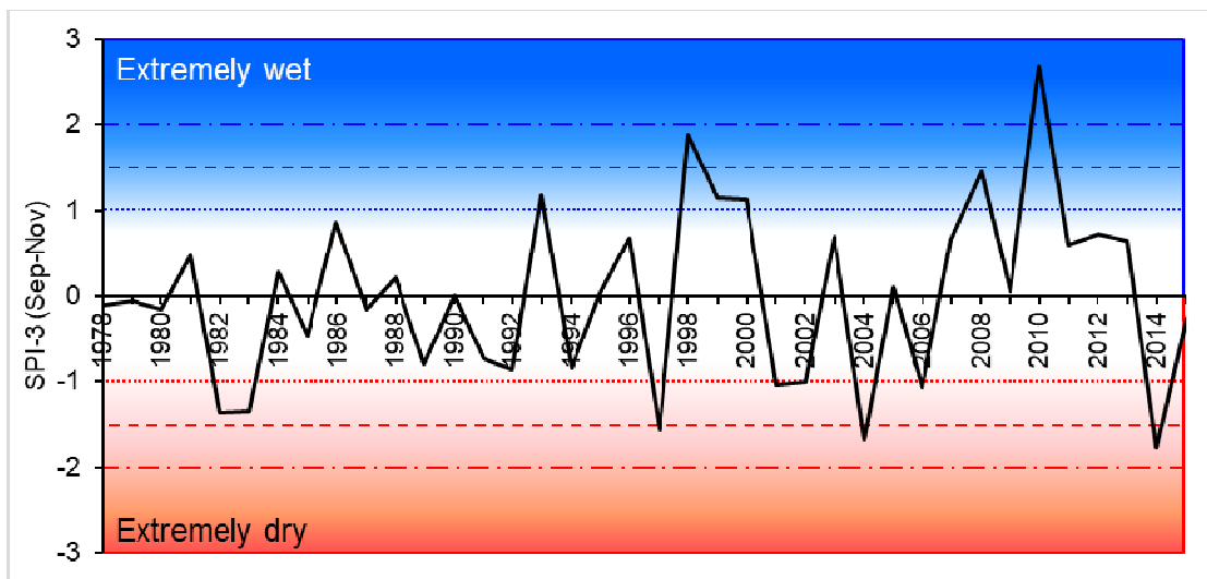
Fig. 3. Variation of dry SPI-9 (a: above) and rainy SPI-3 (b: below) at Phan Rang station, Ninh Thuan province, Vietnam during 1977-2015 (Dot line: Moderately level; Dash line: Severely level; Round dot line: Extremely level)
