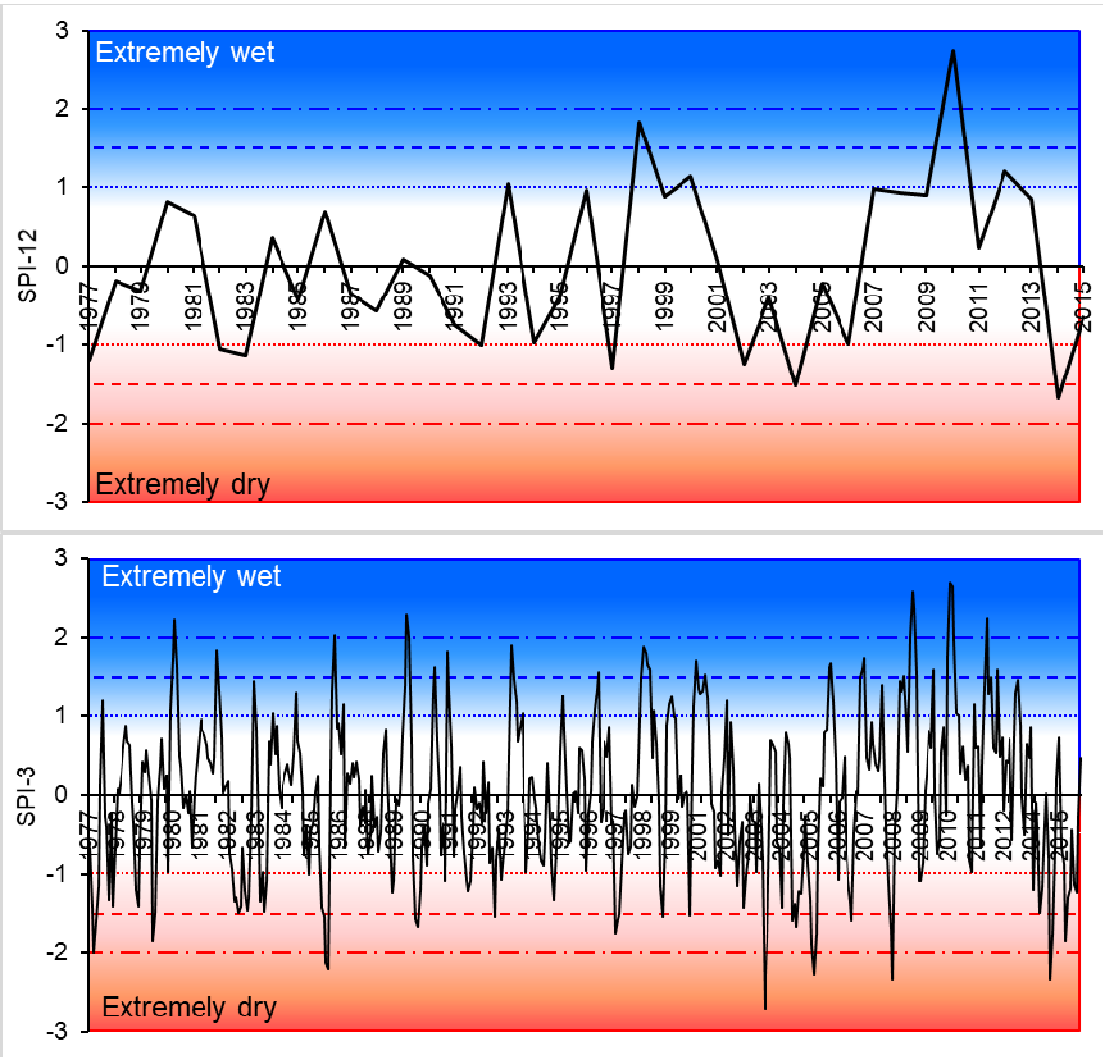
Fig. 2: Variation of annual SPI-12 (a: above) and SPI-3 (b: below) at Phan Rang station, Ninh Thuan province, Vietnam during 1977-2015 (Dot line: Moderately level; Dash line: Severely level; Round dot line: Extremely level)
