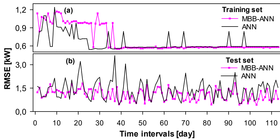
Fig. 9. Cross-validation of one-day forecast
