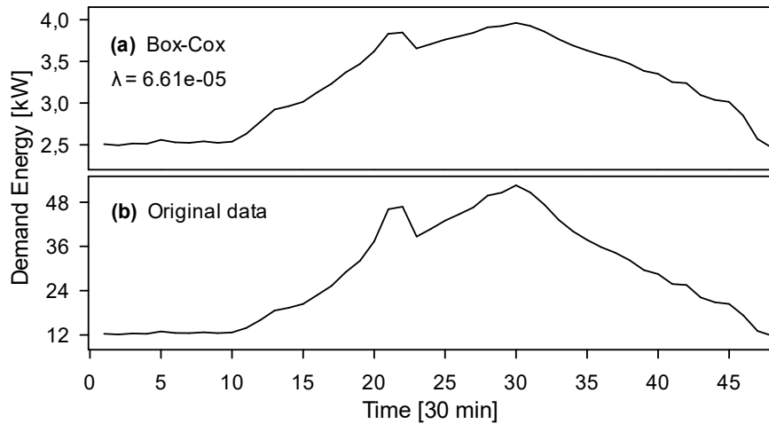
Fig. 5. Example of Box-Cox Transformation
