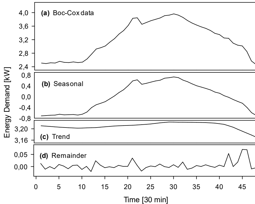
Fig. 6. Example of STL decomposition
