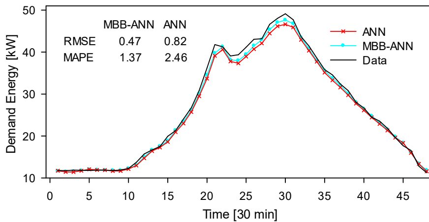
Fig. 4. Forecast one day in advance
