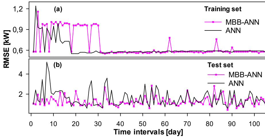
Fig. 10. Cross-validation of two-day forecast
